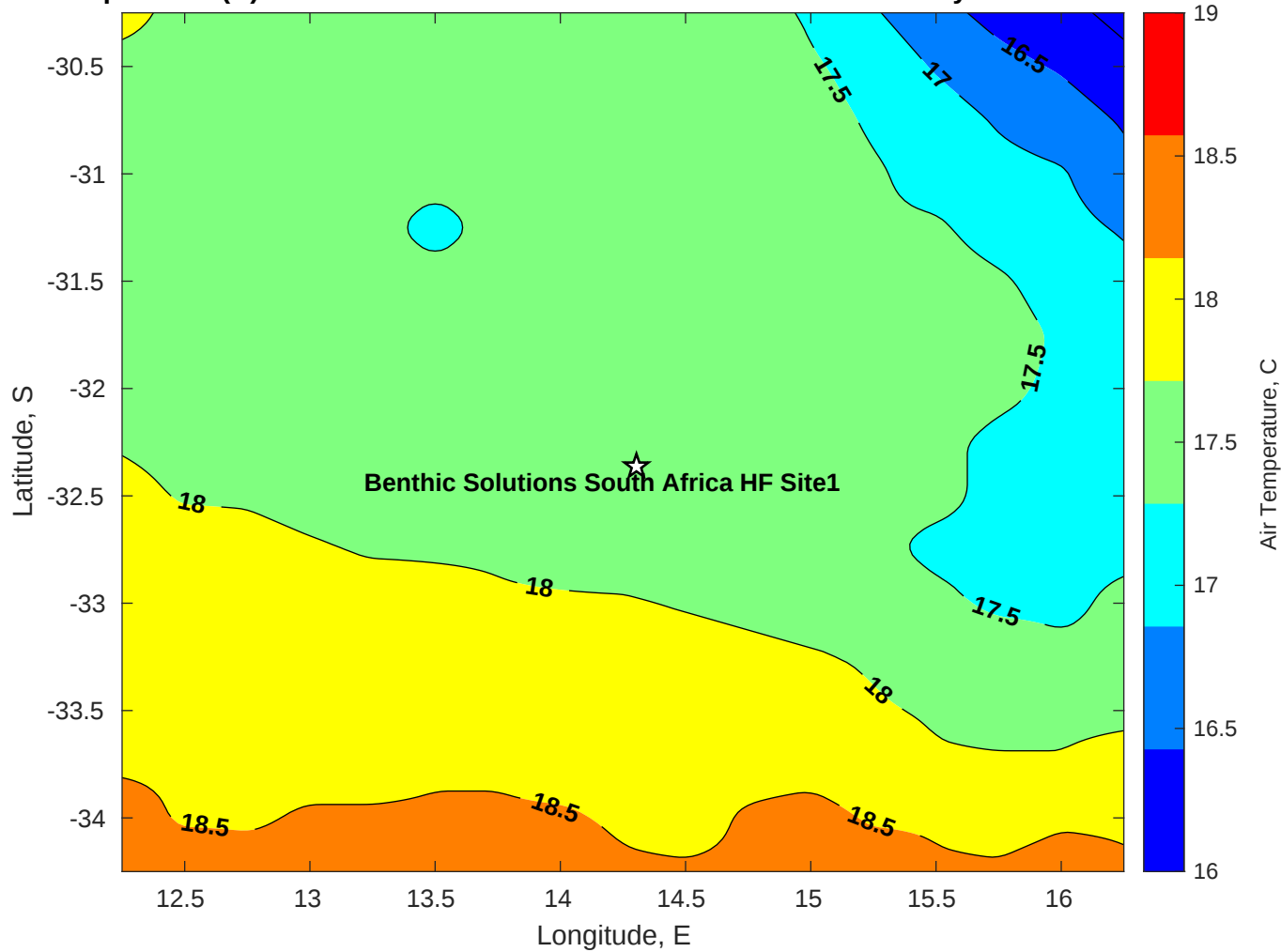
Air Temperature (C) for Benthic Solutions South Africa HF Site1 at 10-May-2025
