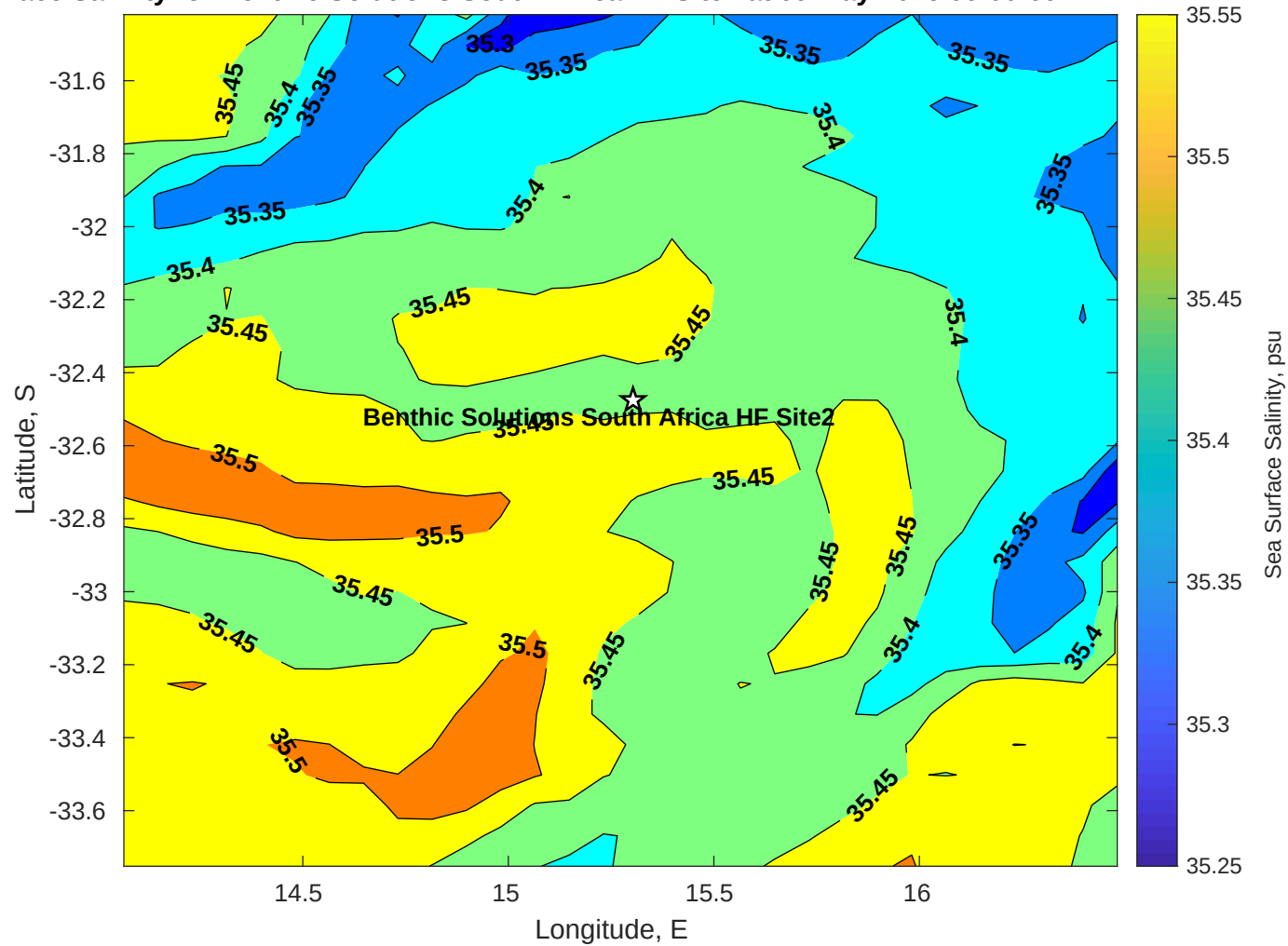
Surface Salinity for Benthic Solutions South Africa HF Site2 at 09-May-2025 00:00:00
