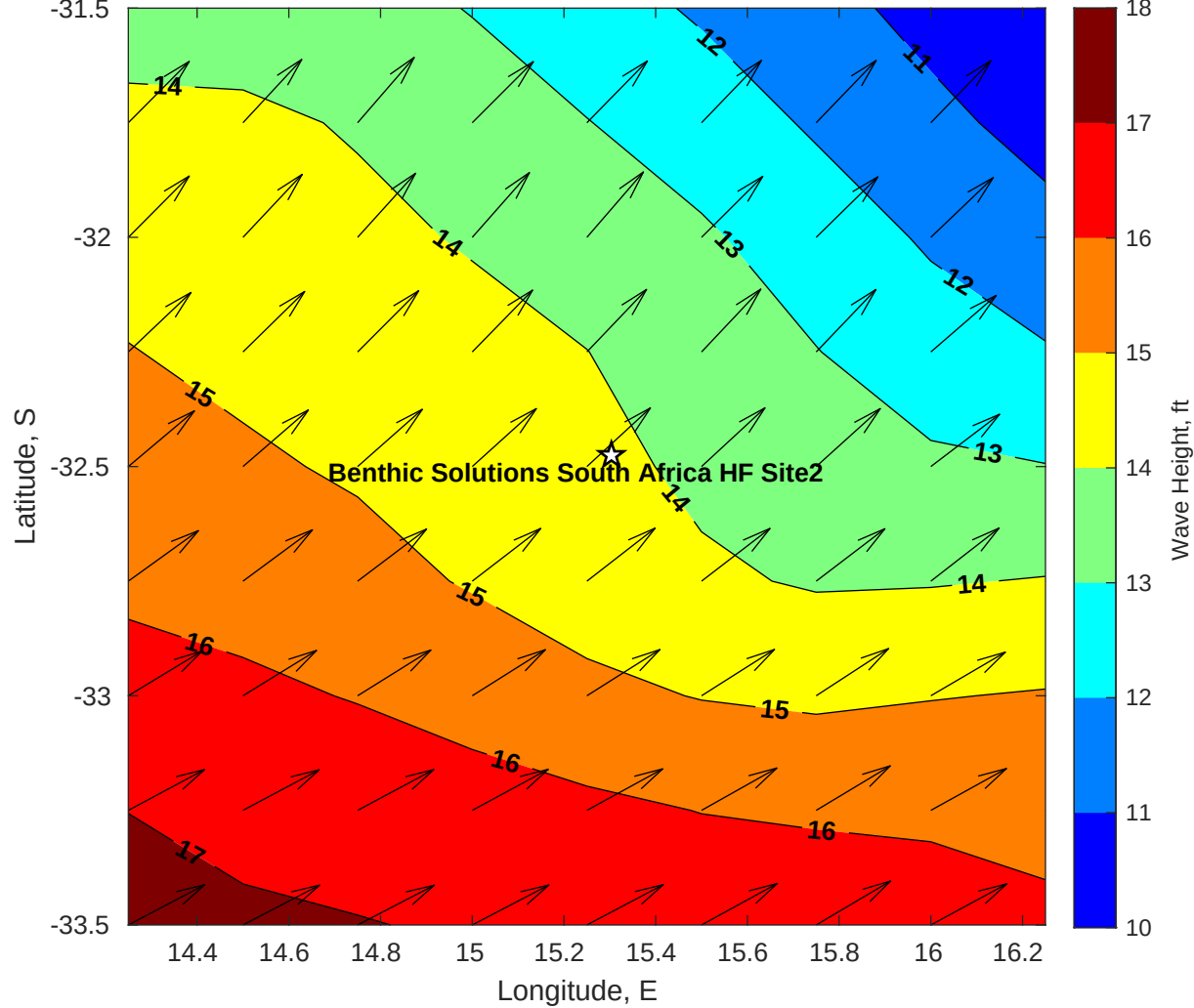
Wave Height (ft) for Benthic Solutions South Africa HF Site2 at 10-May-2025 09:00:00
