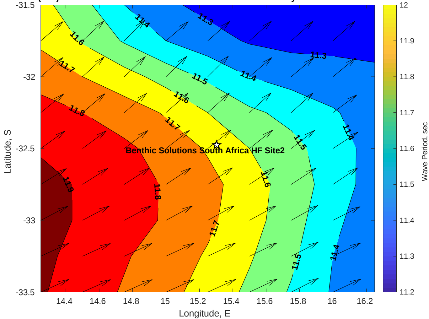
Wave Period (sec) for Benthic Solutions South Africa HF Site2 at 10-May-2025 09:00:00
