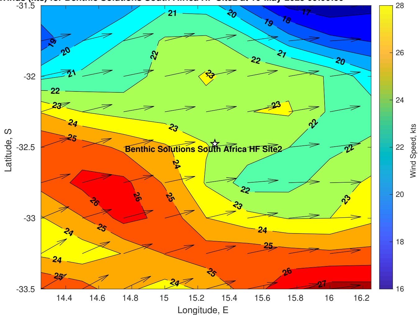
Winds (kts) for Benthic Solutions South Africa HF Site2 at 10-May-2025 09:00:00
