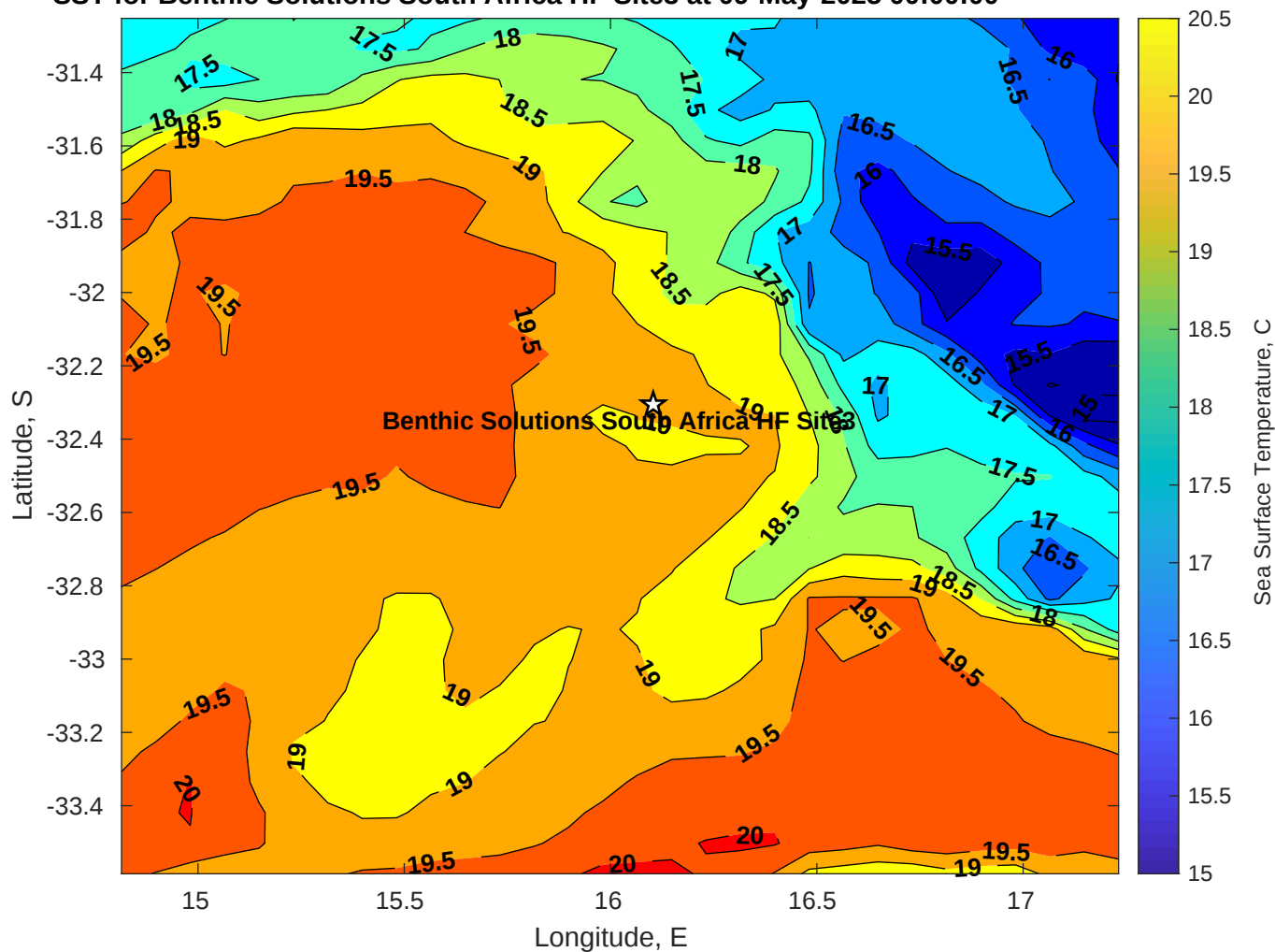
SST for Benthic Solutions South Africa HF Site3 at 09-May-2025 00:00:00
