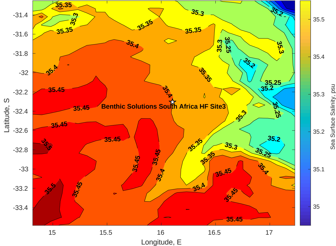
Surface Salinity for Benthic Solutions South Africa HF Site3 at 09-May-2025 00:00:00
