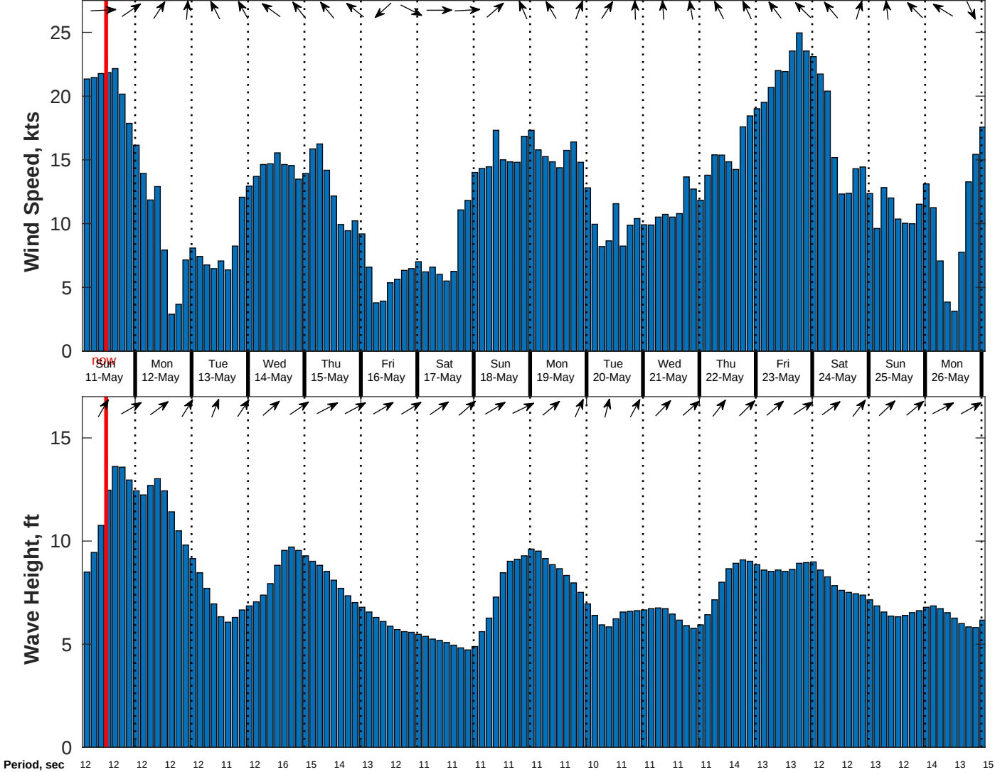
Wind & Wave Forecast for Benthic Solutions South Africa HF Site3 from 10-May-2025 02:00:00 to 26-May-2025 02:00:00
