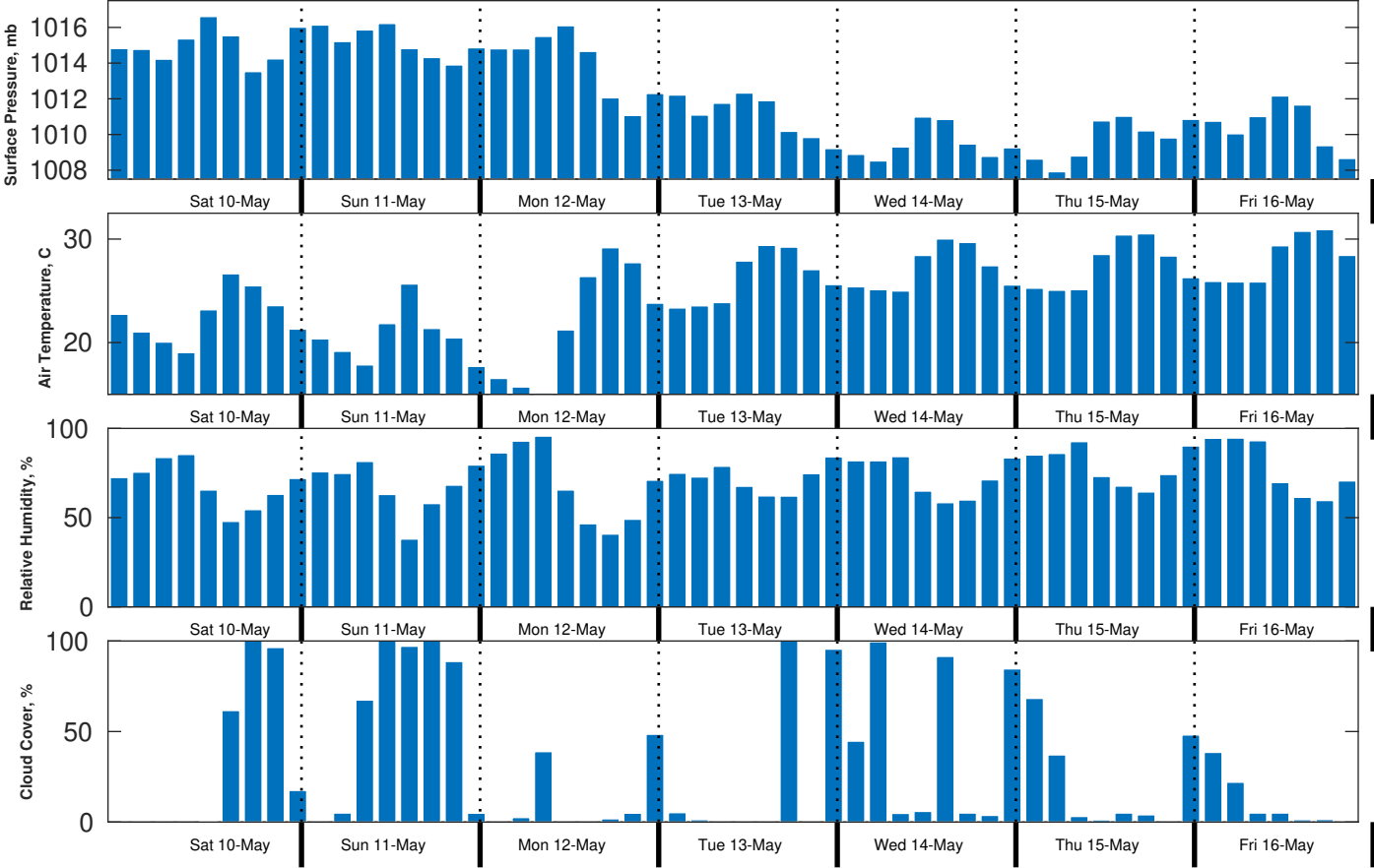
Met Forecast for Brooks McCall from 10-May-2025 00:00:00 to 17-May-2025 00:00:00
