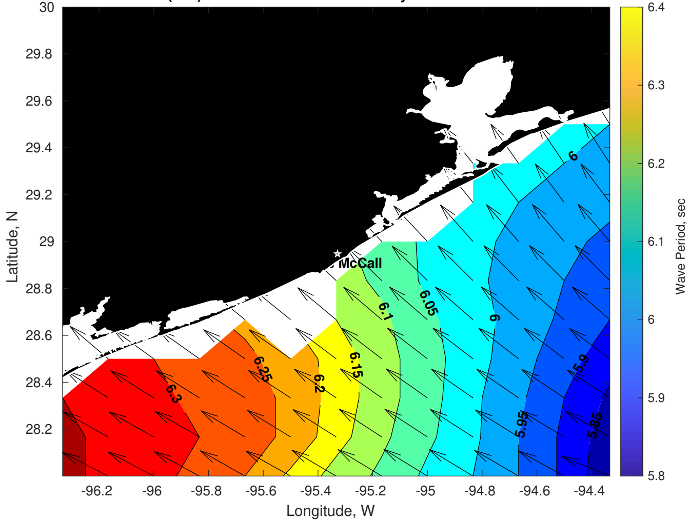
Wave Period (sec) for Brooks McCall at 10-May-2025 09:00:00
