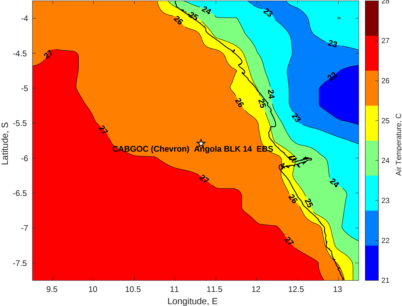
Air Temperature (C) for CABGOC (Chevron) Angola BLK 14 EBS at 10-May-2025
