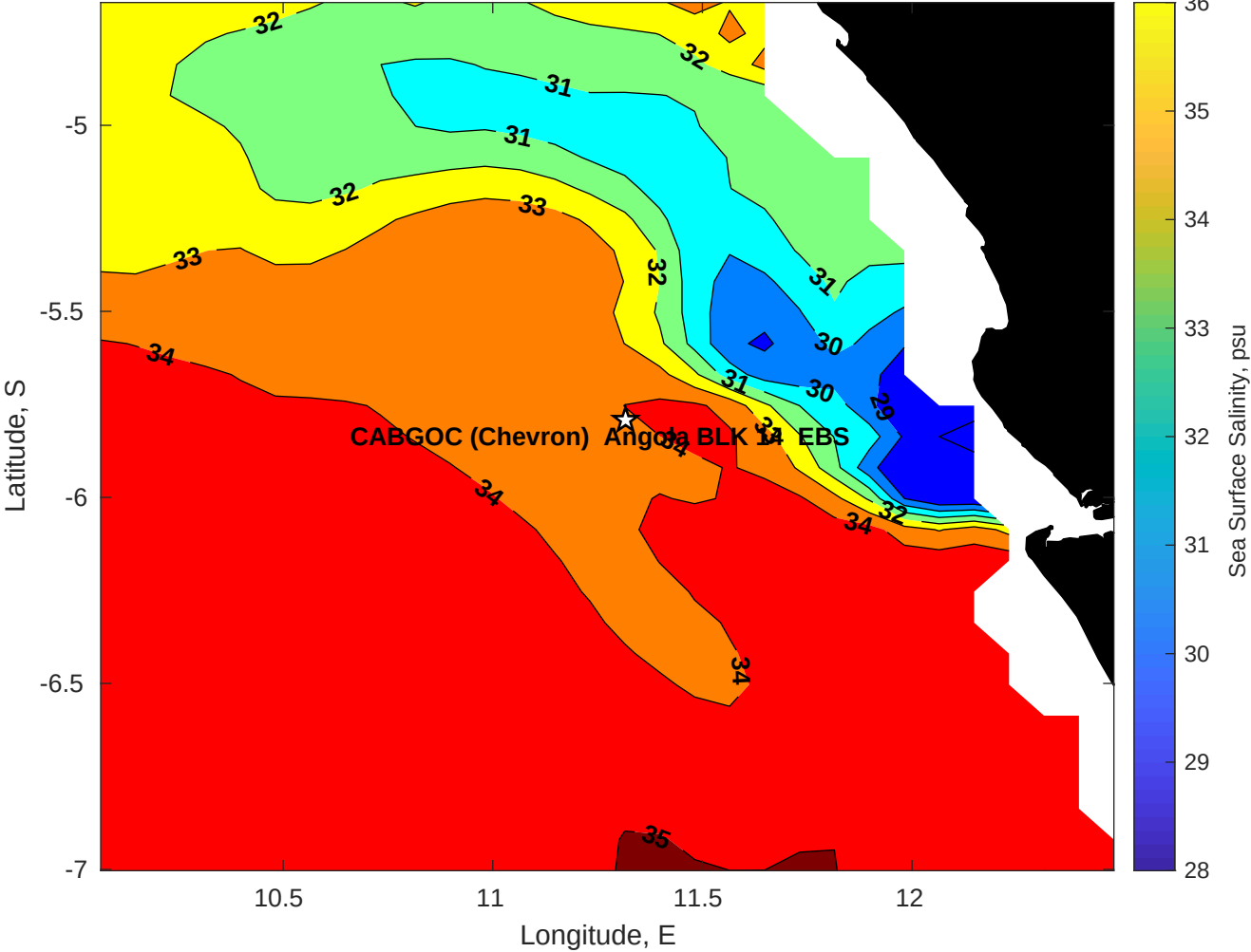
Surface Salinity for CABGOC (Chevron) Angola BLK 14 EBS at 09-May-2025 00:00:00
