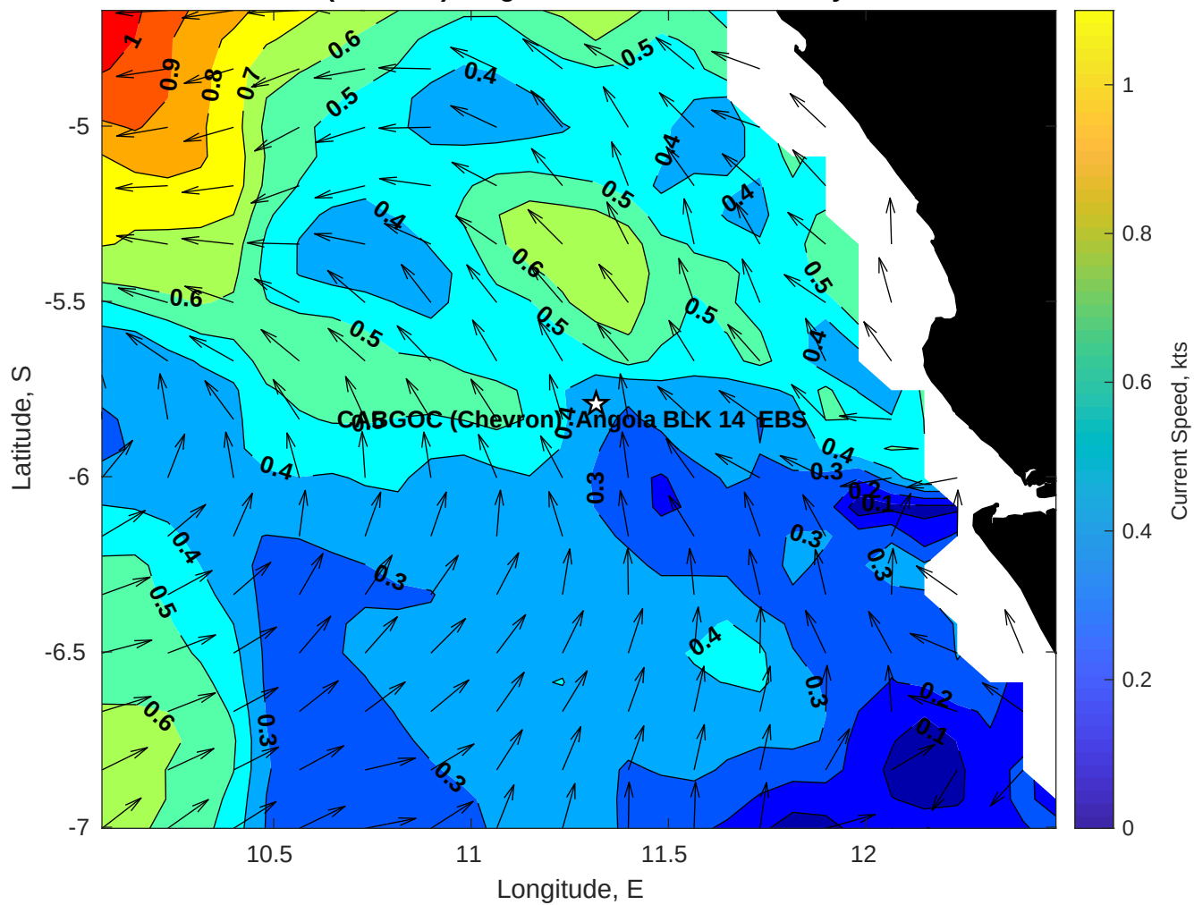
Surface Currents for CABGOC (Chevron) Angola BLK 14 EBS at 09-May-2025 00:00:00
