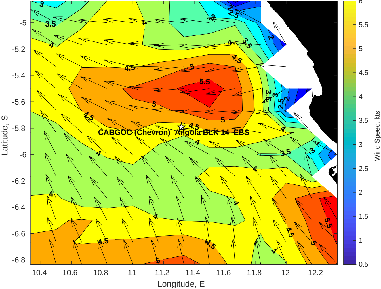
Winds (kts) for CABGOC (Chevron) Angola BLK 14 EBS at 10-May-2025 09:00:00
