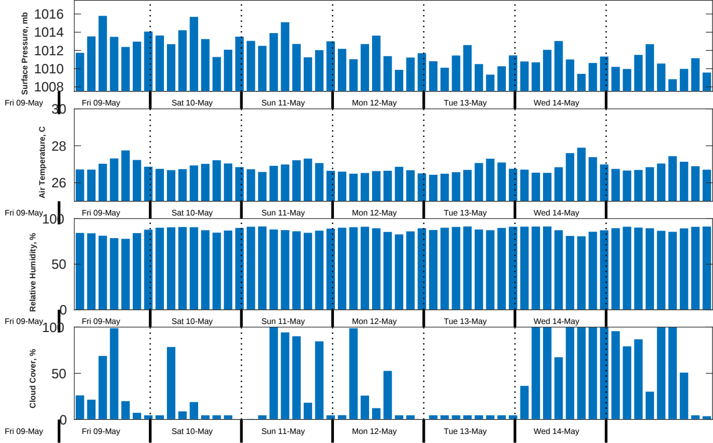
Met Forecast for CABGOC (Chevron) Angola BLK 14 EBS from 10-May-2025 00:00:00 to 17-May-2025 00:00:00
