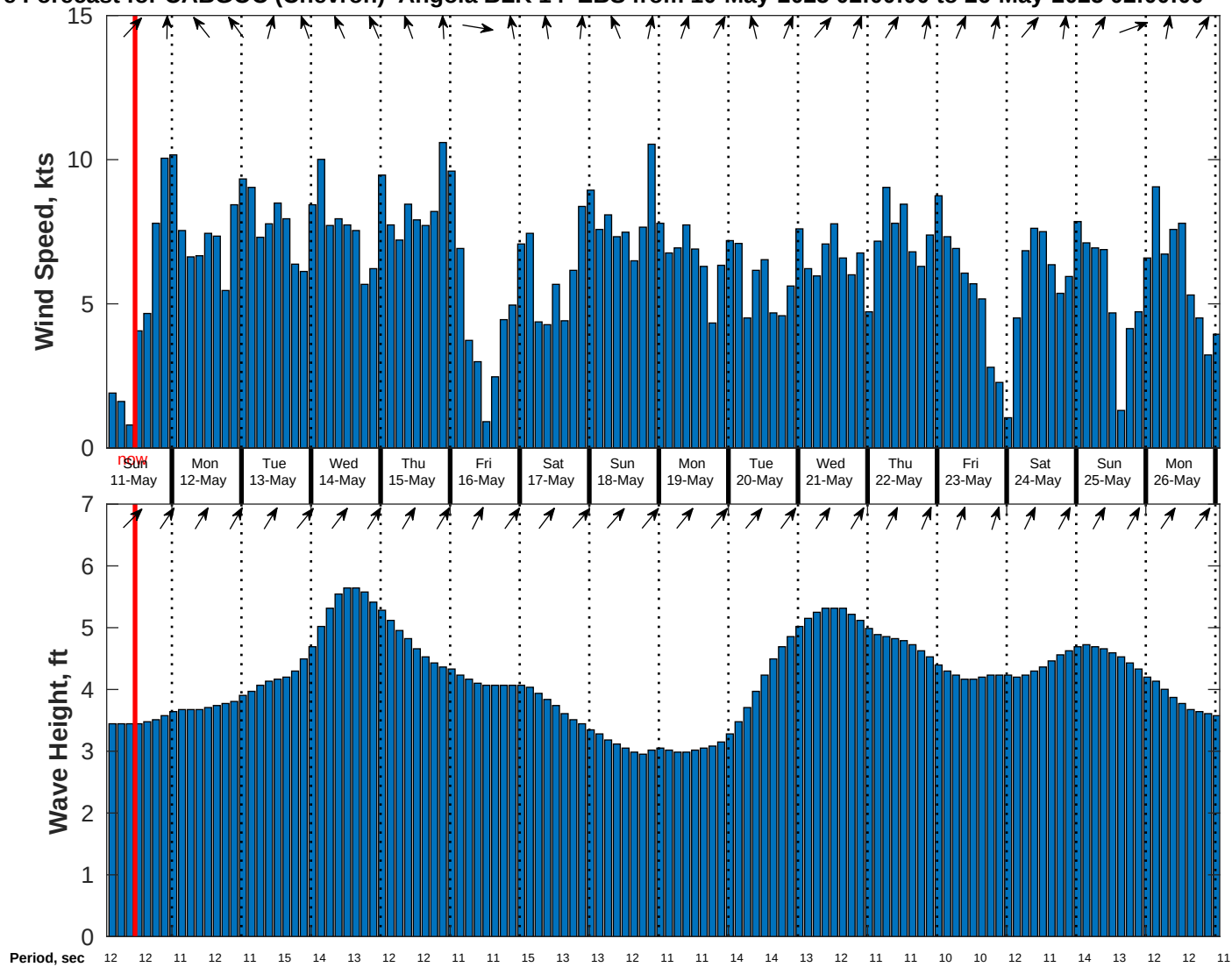
Wind & Wave Forecast for CABGOC (Chevron) Angola BLK 14 EBS from 10-May-2025 02:00:00 to 26-May-2025 02:00:00
