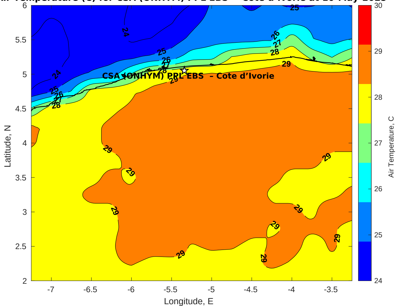
Air Temperature (C) for CSA (ONHYM) PPL EBS - Cote d'Ivoire at 10-May-2025
