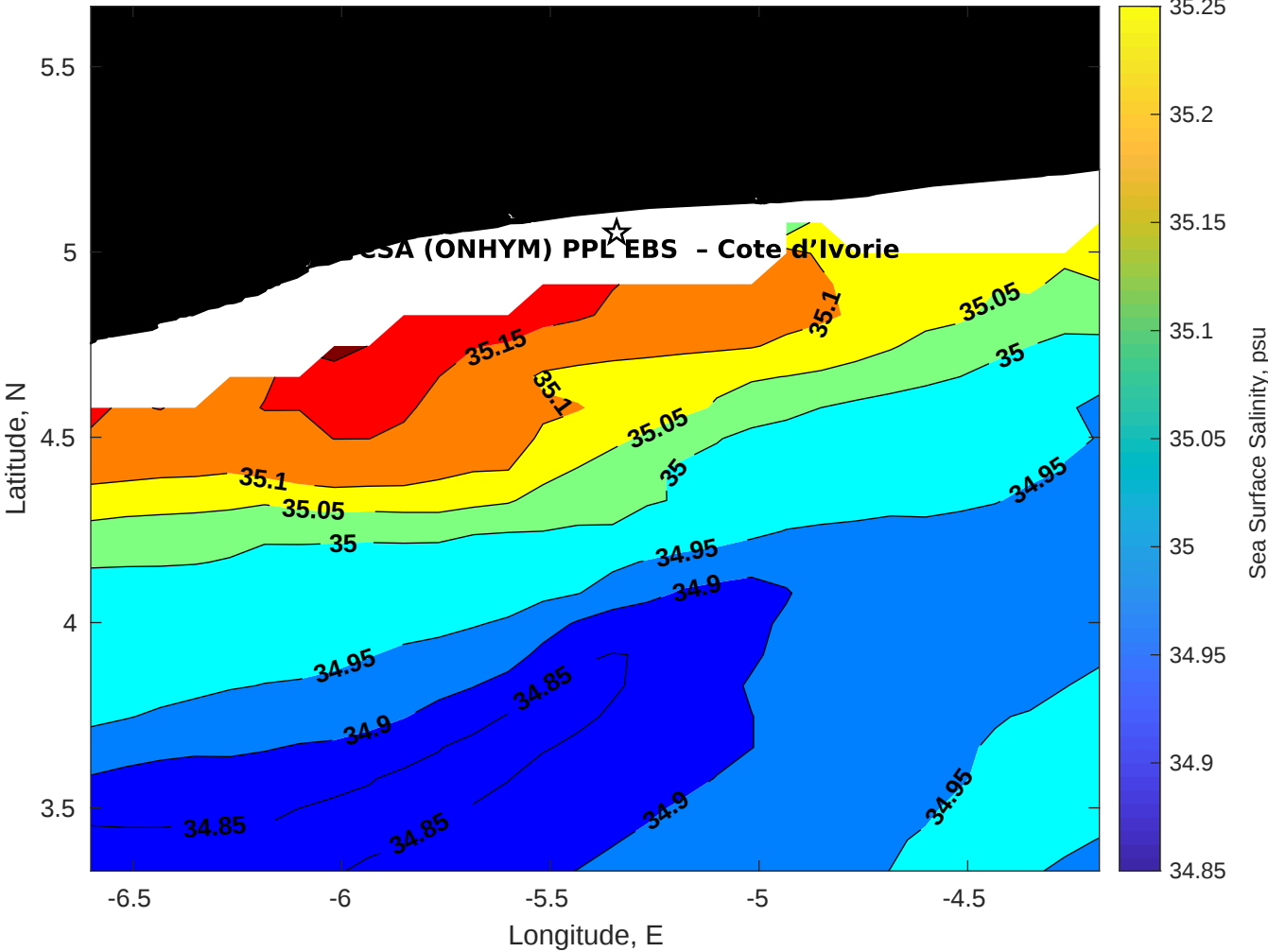
Surface Salinity for CSA (ONHYM) PPL EBS - Cote d'Ivoire at 09-May-2025 00:00:00
