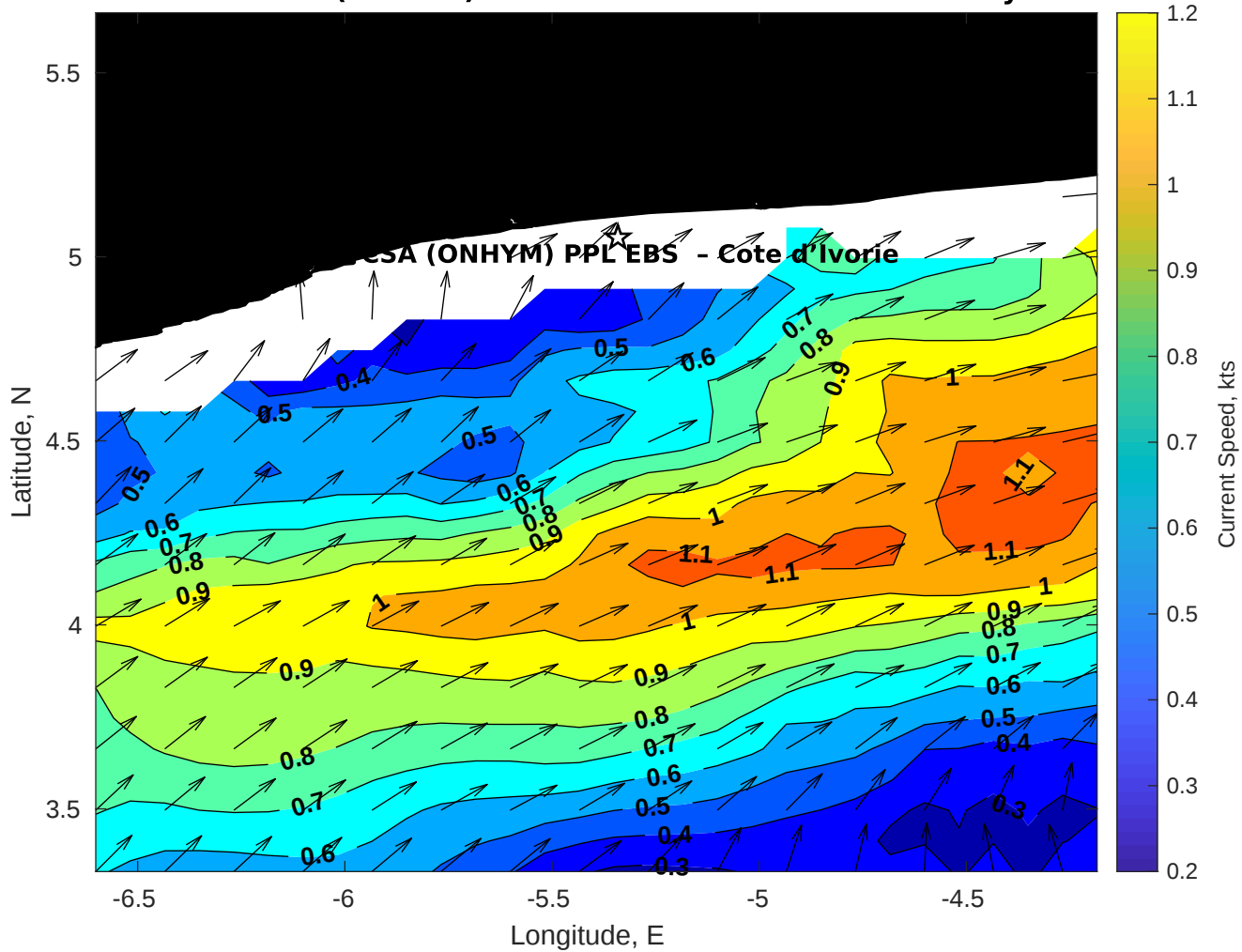
Surface Currents for CSA (ONHYM) PPL EBS - Cote d'Ivoire at 09-May-2025 00:00:00
