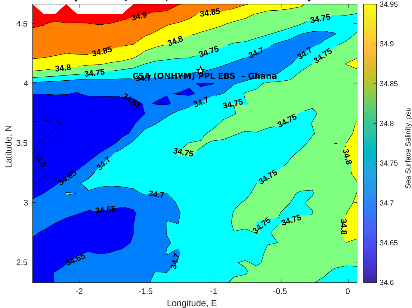
Surface Salinity for CSA (ONHYM) PPL EBS - Ghana at 09-May-2025 00:00:00
