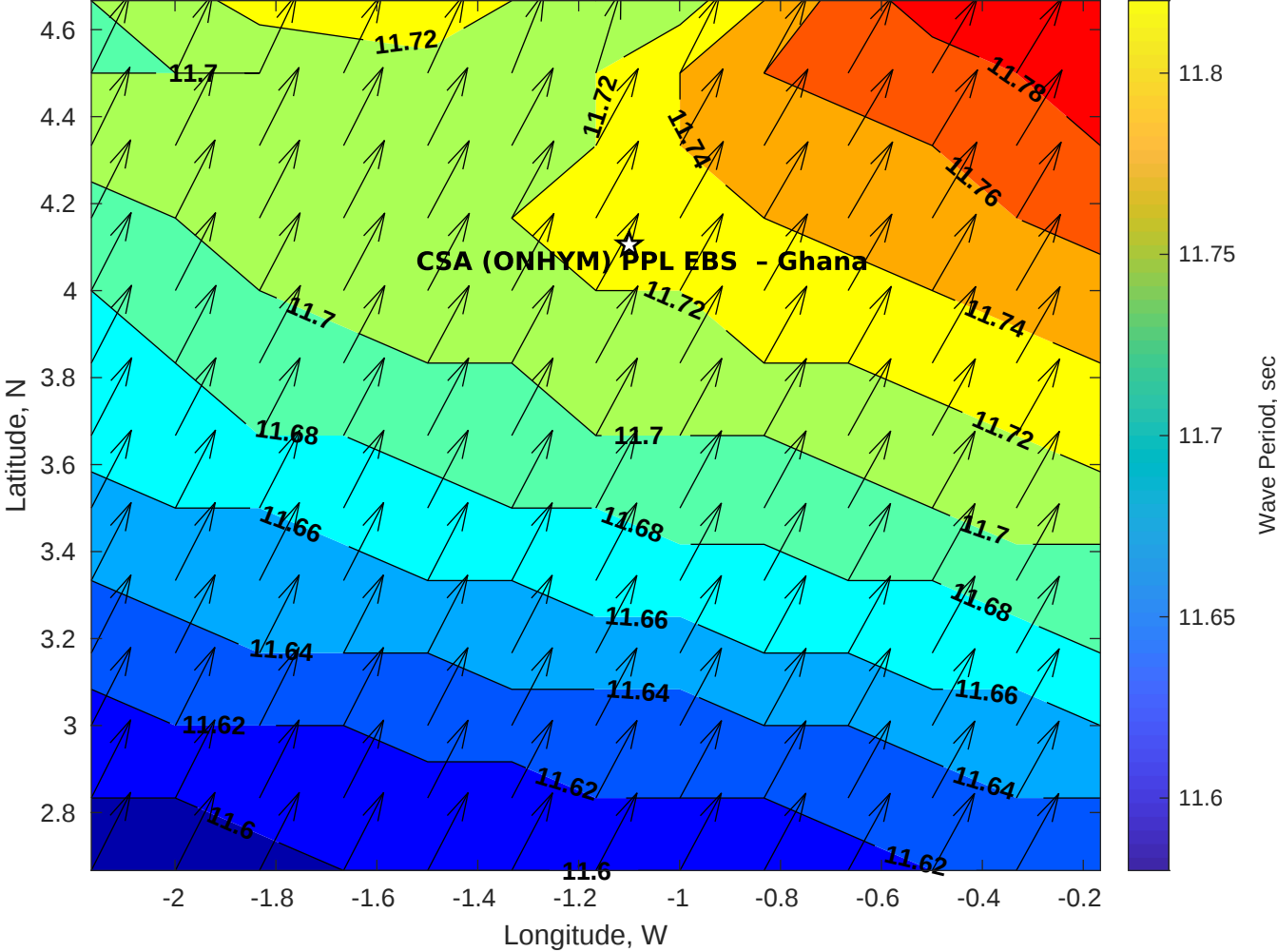
Wave Period (sec) for CSA (ONHYM) PPL EBS - Ghana at 10-May-2025 09:00:00
