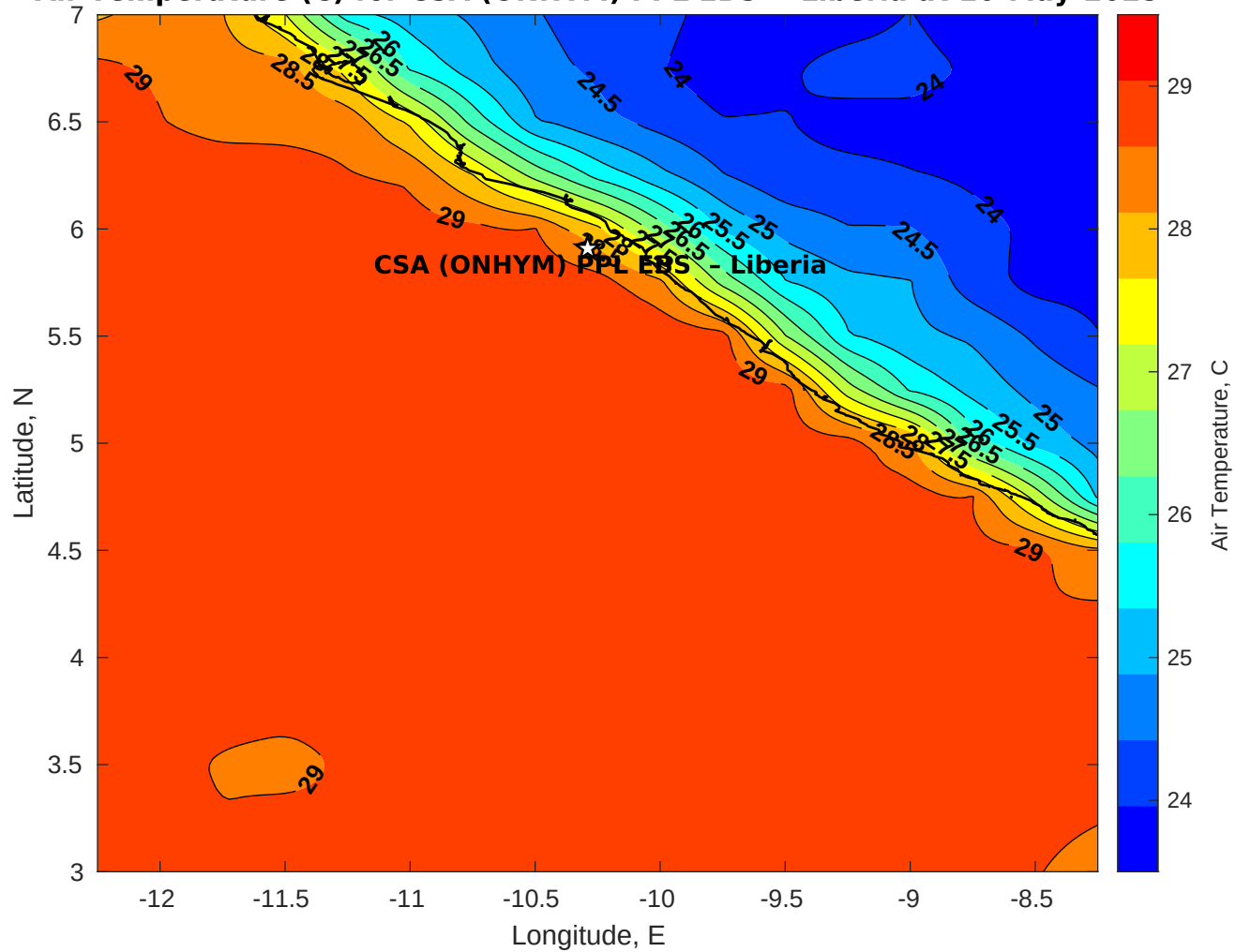
Air Temperature (C) for CSA (ONHYM) PPL EBS - Liberia at 10-May-2025
