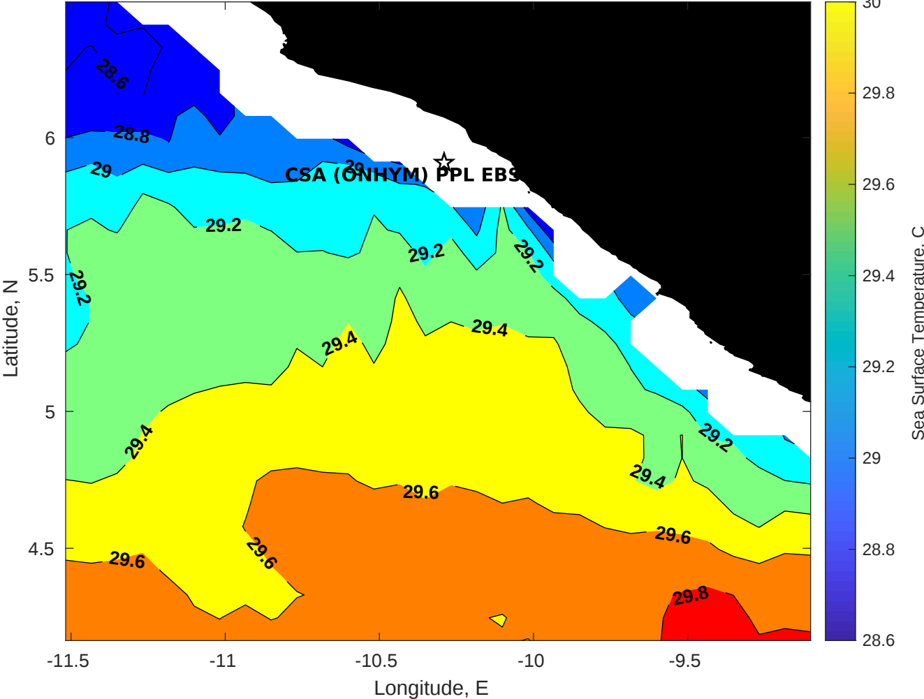
SST for CSA (ONHYM) PPL EBS - Liberia at 09-May-2025 00:00:00
