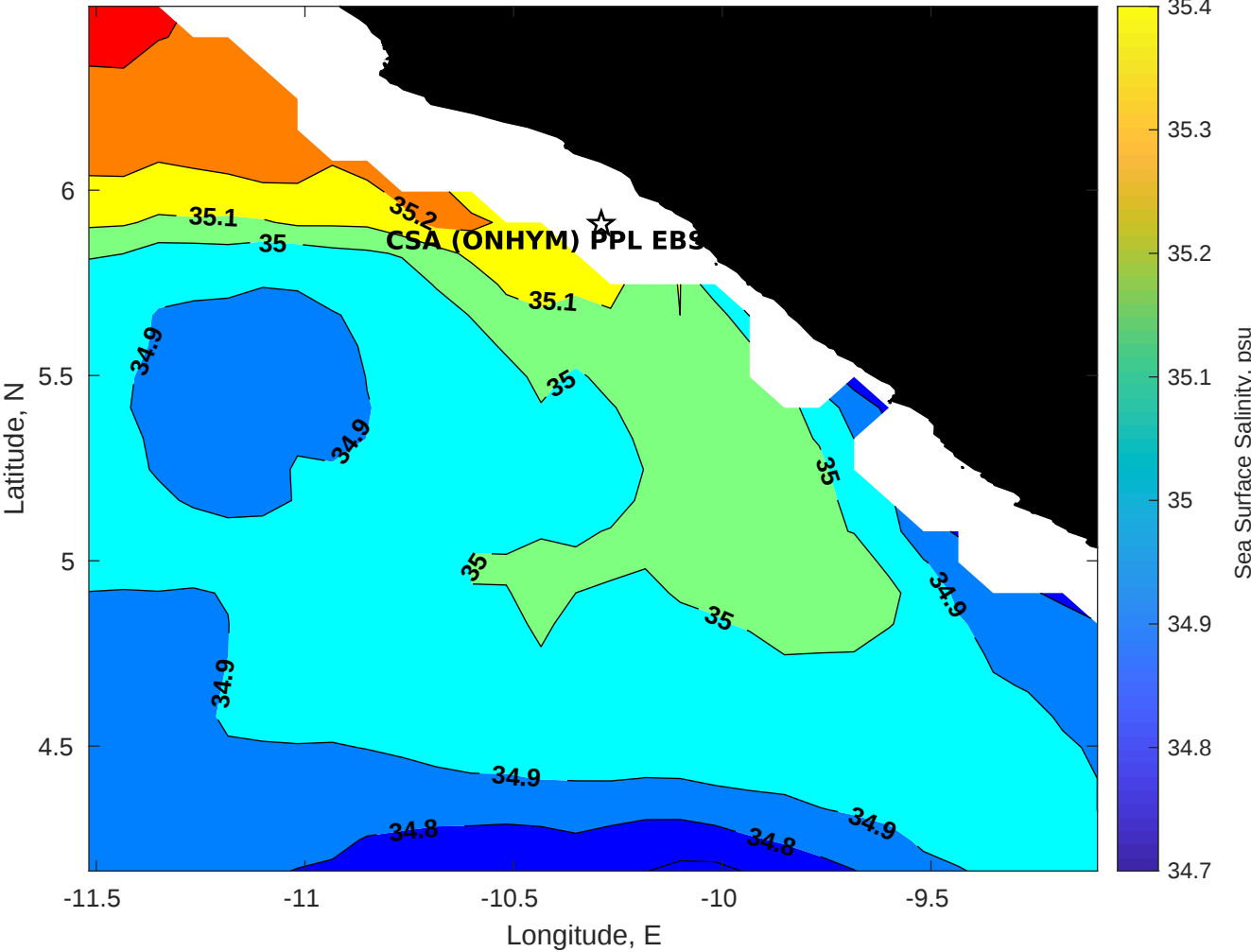
Surface Salinity for CSA (ONHYM) PPL EBS - Liberia at 09-May-2025 00:00:00
