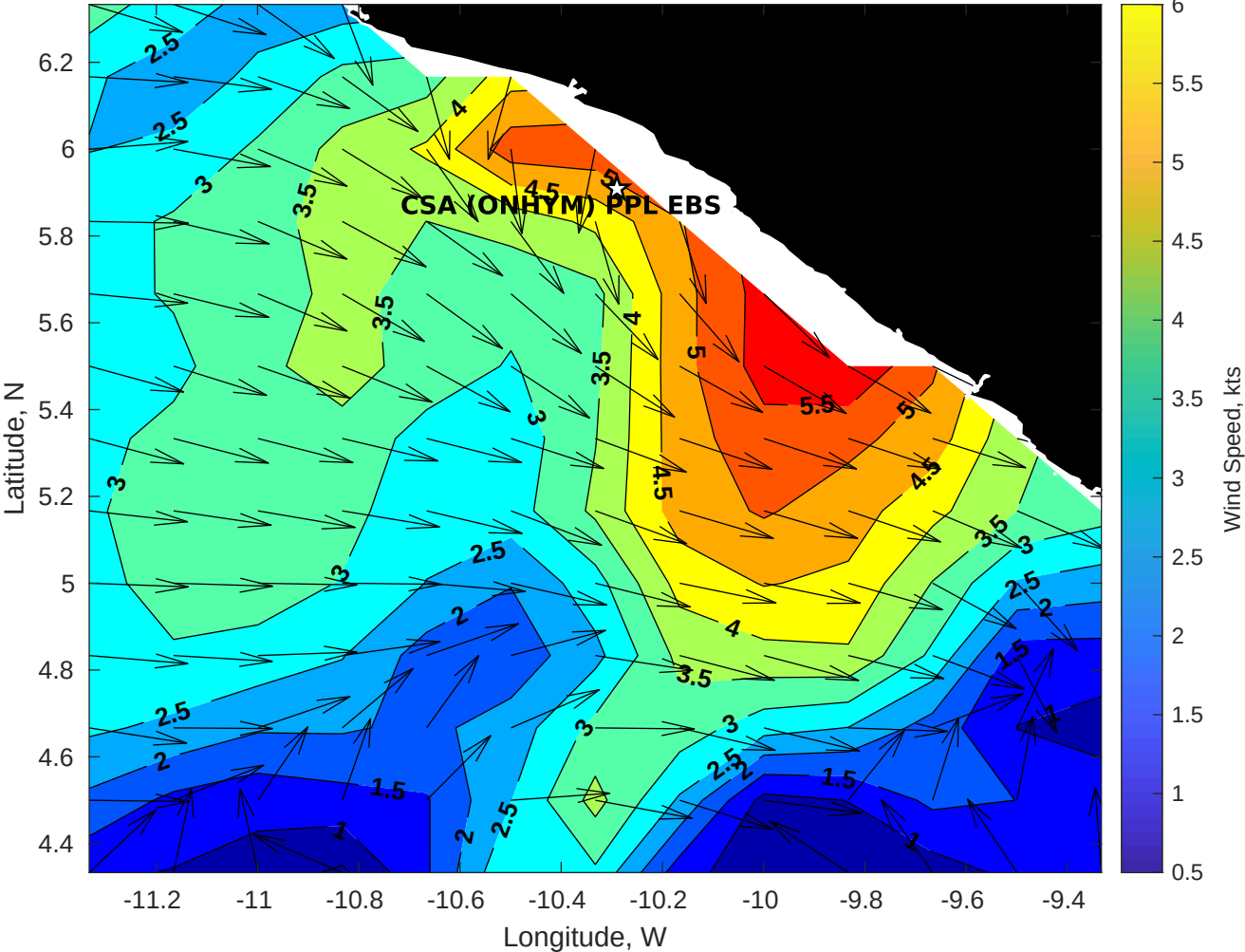
Winds (kts) for CSA (ONHYM) PPL EBS - Liberia at 10-May-2025 09:00:00
