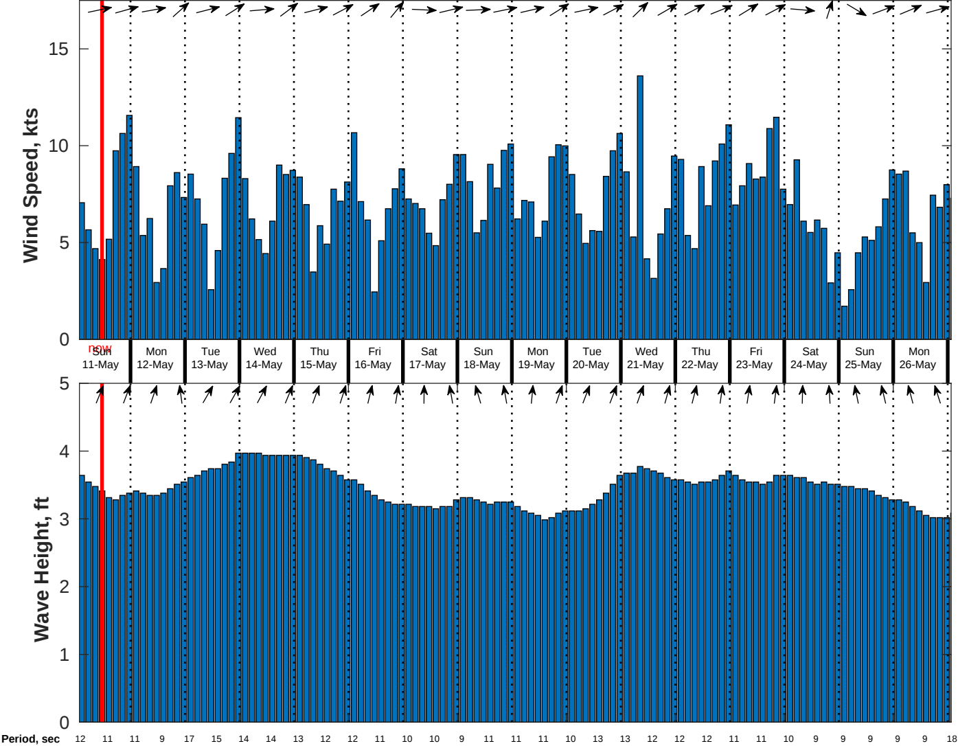
Wind & Wave Forecast for CSA (ONHYM) PPL EBS - Liberia from 10-May-2025 01:00:00 to 26-May-2025 01:00:00
