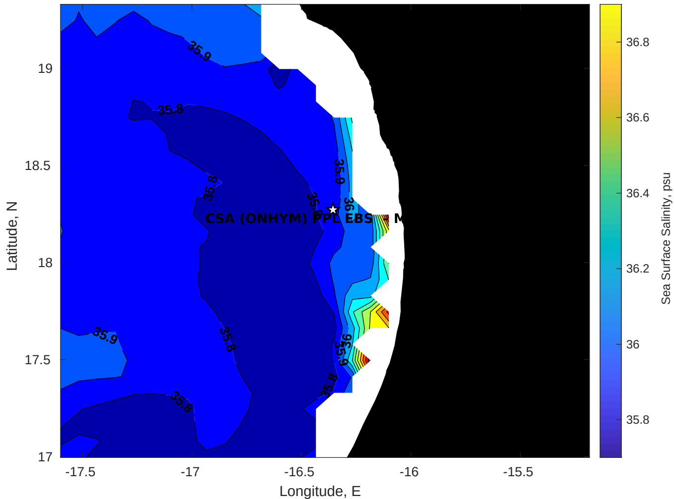
Surface Salinity for CSA (ONHYM) PPL EBS - Mauritania at 09-May-2025 00:00:00
