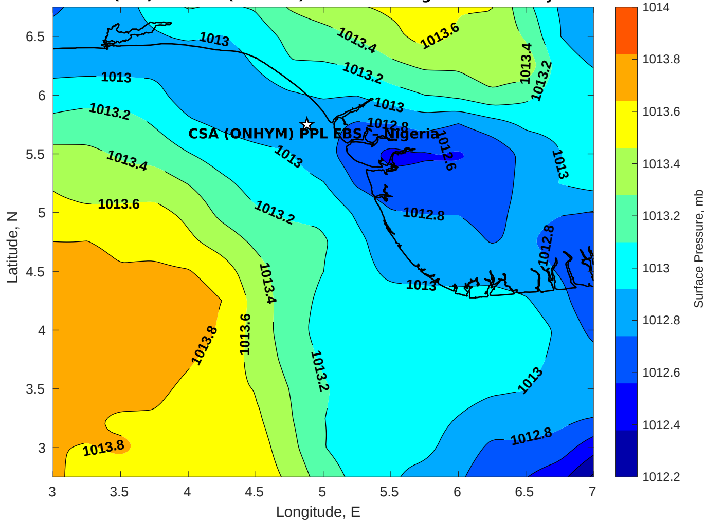
Surface Pressure (mb) for CSA (ONHYM) PPL EBS - Nigeria at 12-May-2025 00:00:00
