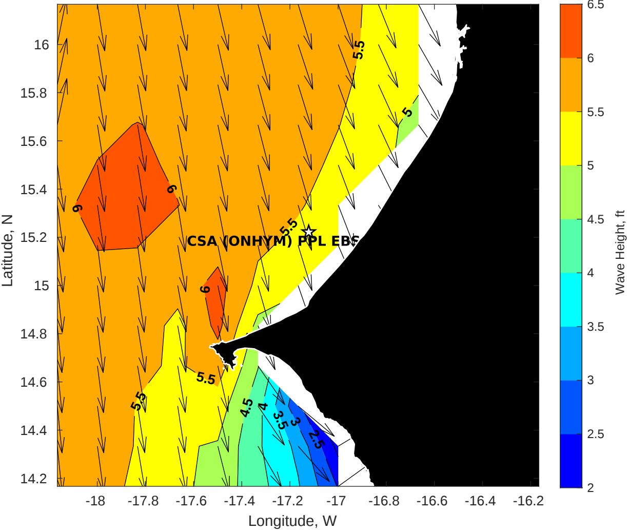
Wave Height (ft) for CSA (ONHYM) PPL EBS - Senegal at 10-May-2025 09:00:00
