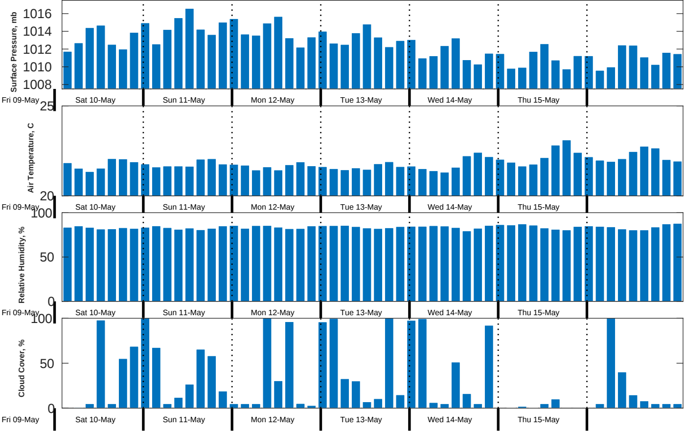
Met Forecast for CSA (ONHYM) PPL EBS - Senegal from 10-May-2025 00:00:00 to 17-May-2025 00:00:00
