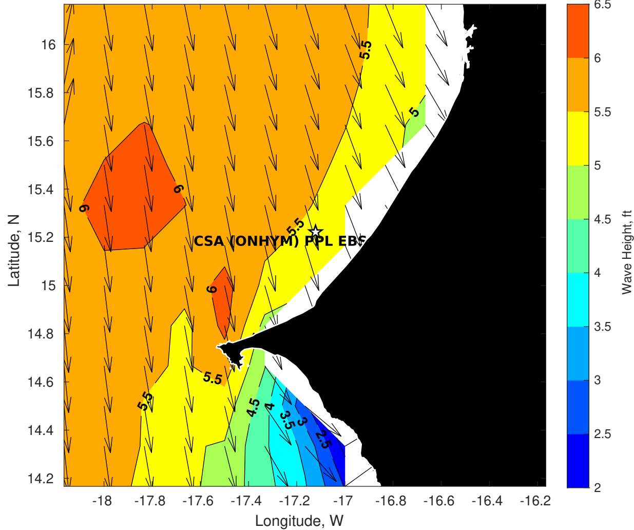
Wave Height (ft) for CSA (ONHYM) PPL EBS - Senegal at 10-May-2025 09:00:00
