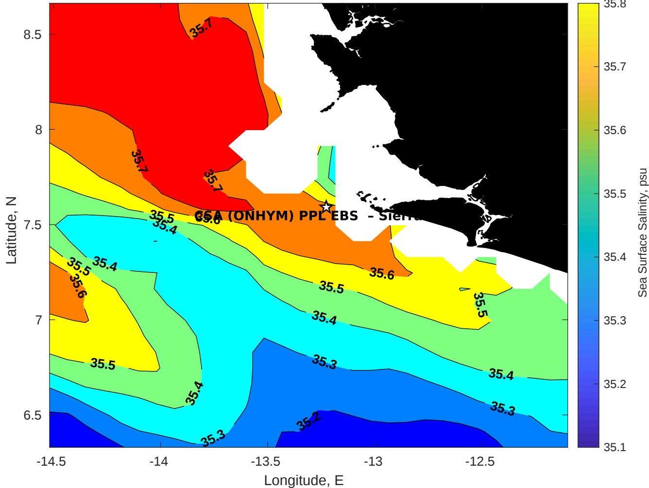
Surface Salinity for CSA (ONHYM) PPL EBS - Sierra Leone at 09-May-2025 00:00:00
