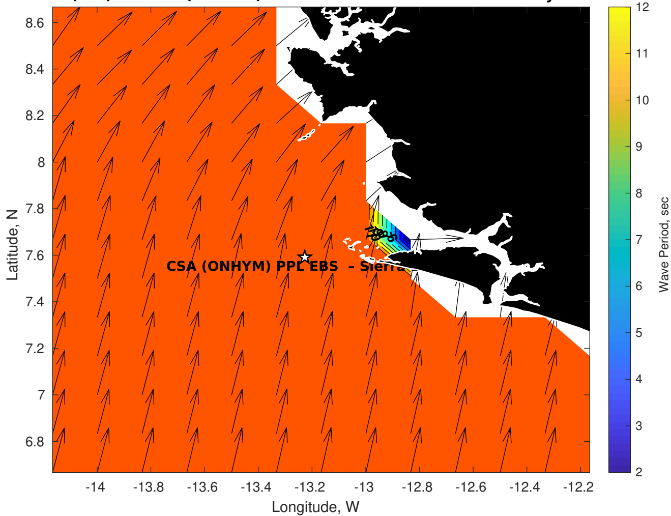
Wave Period (sec) for CSA (ONHYM) PPL EBS - Sierra Leone at 10-May-2025 09:00:00
