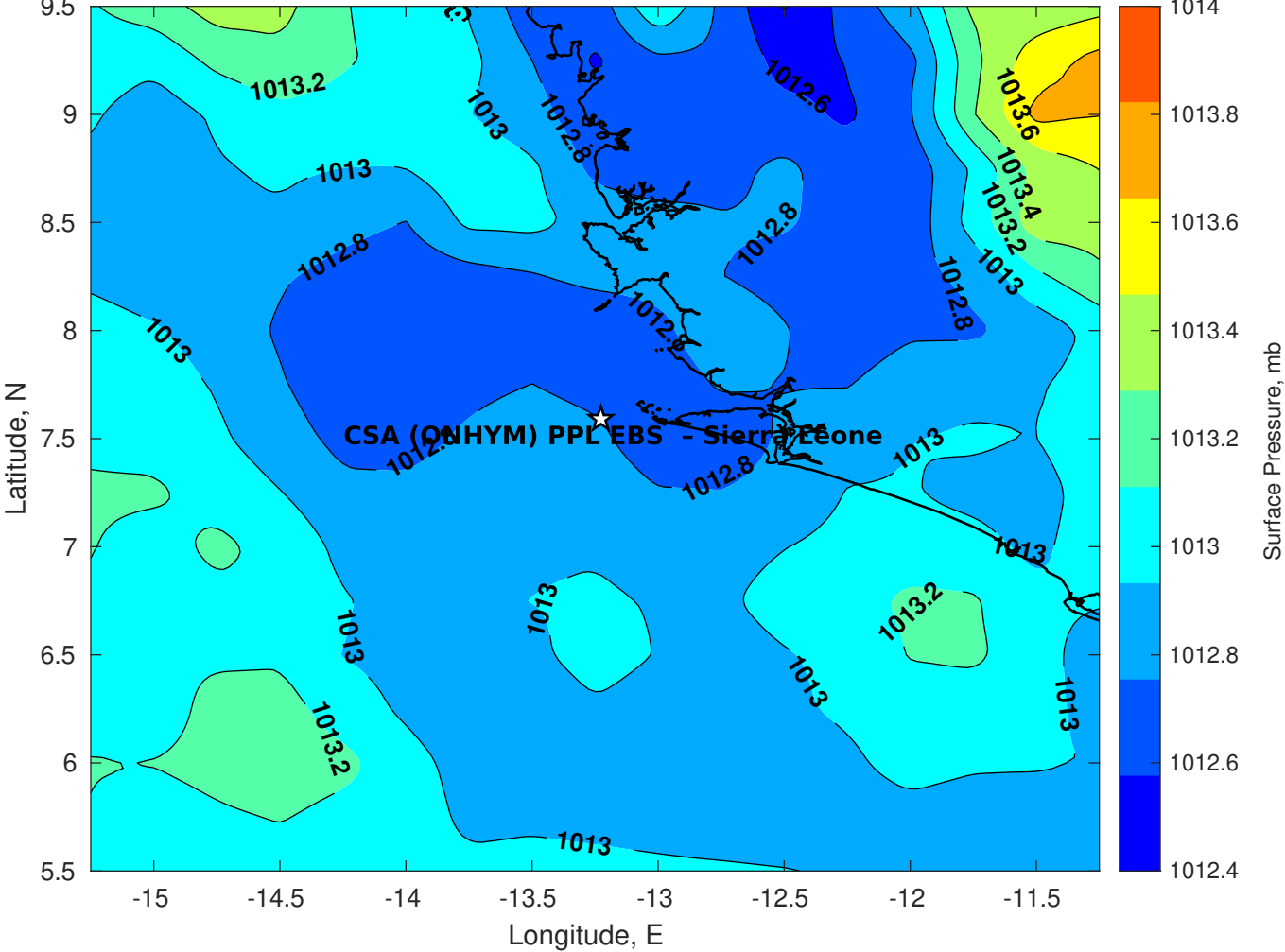
Surface Pressure (mb) for CSA (ONHYM) PPL EBS - Sierra Leone at 10-May-2025 00:00:00
