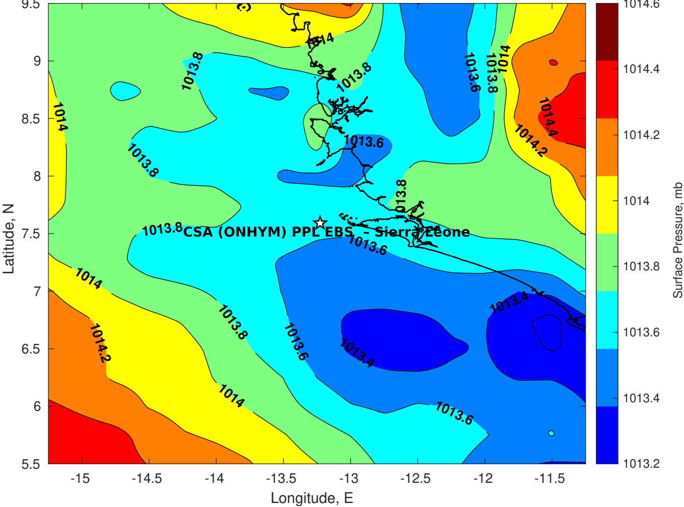
Surface Pressure (mb) for CSA (ONHYM) PPL EBS - Sierra Leone at 11-May-2025 00:00:00
