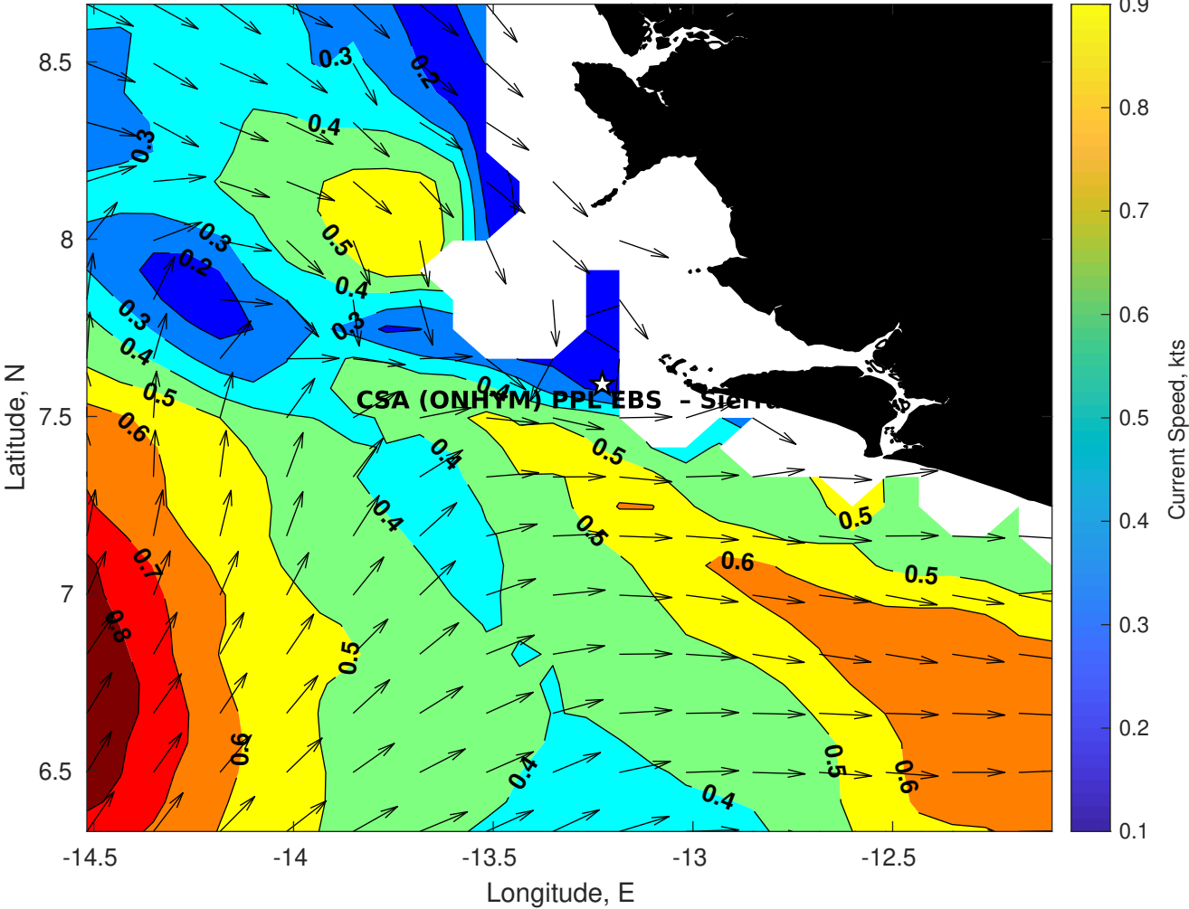
Surface Currents for CSA (ONHYM) PPL EBS - Sierra Leone at 09-May-2025 00:00:00
