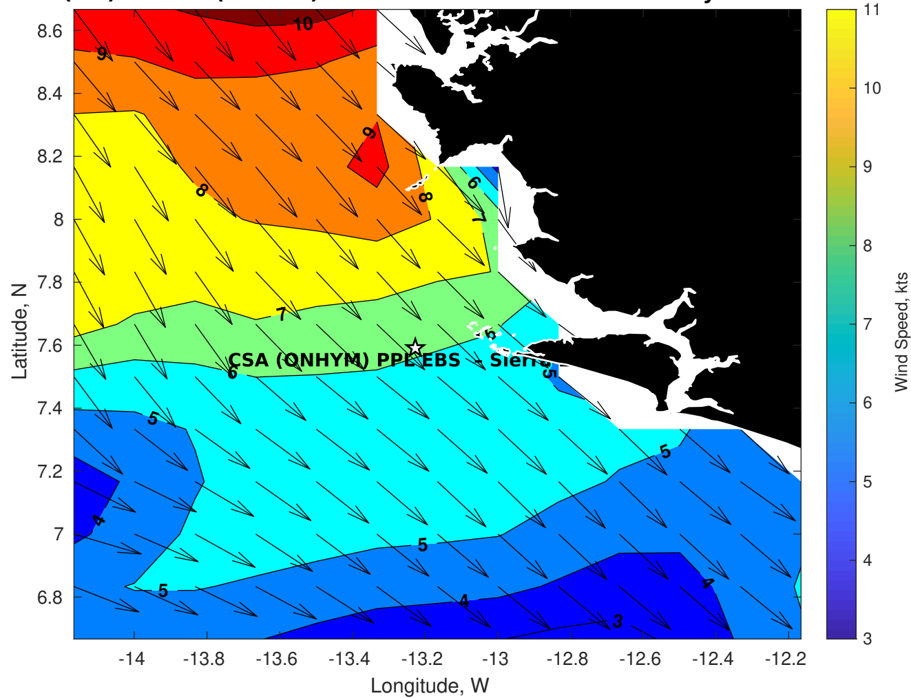
Winds (kts) for CSA (ONHYM) PPL EBS - Sierra Leone at 10-May-2025 09:00:00
