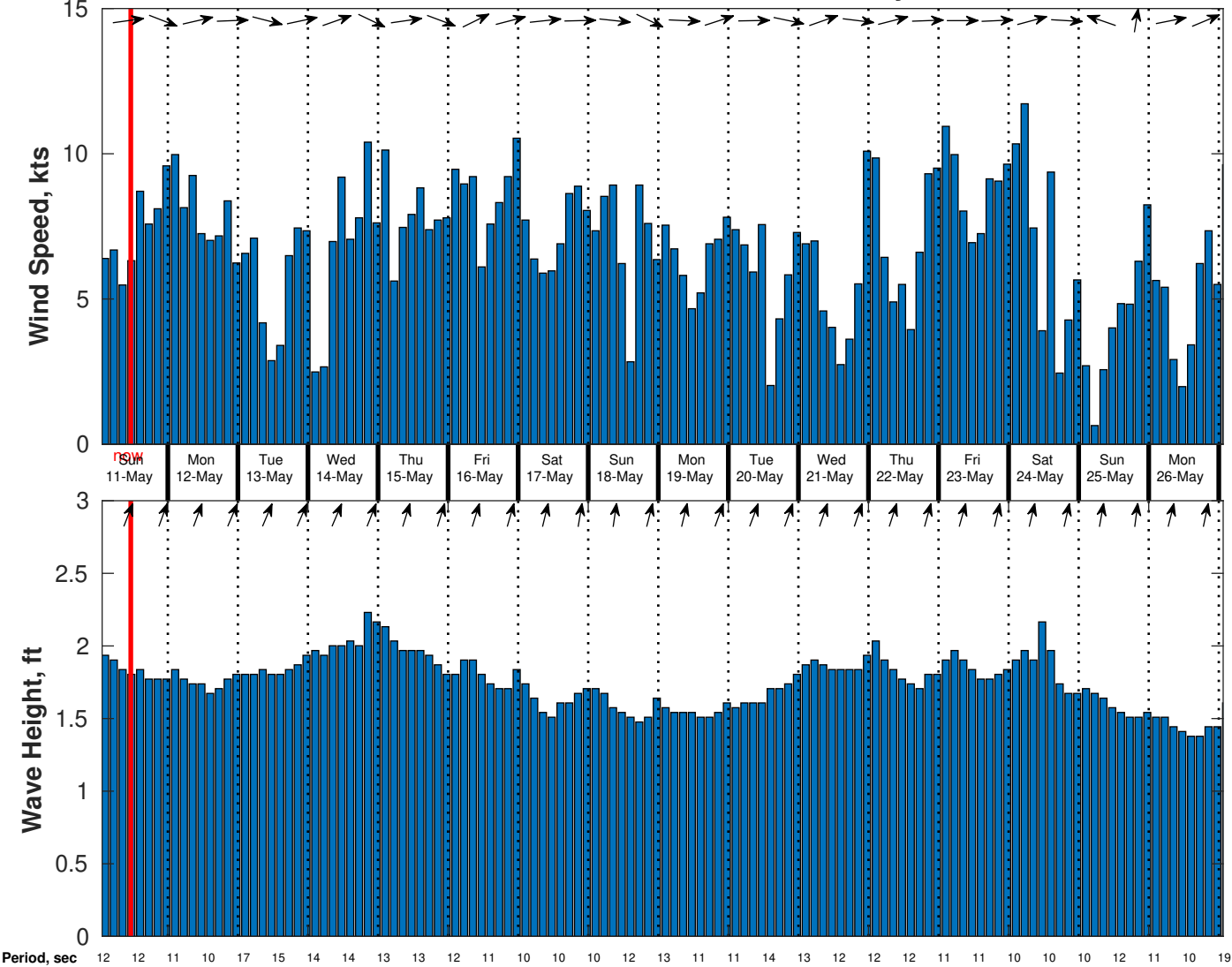
Wind & Wave Forecast for CSA (ONHYM) PPL EBS - Sierra Leone from 10-May-2025 01:00:00 to 26-May-2025 01:00:00
