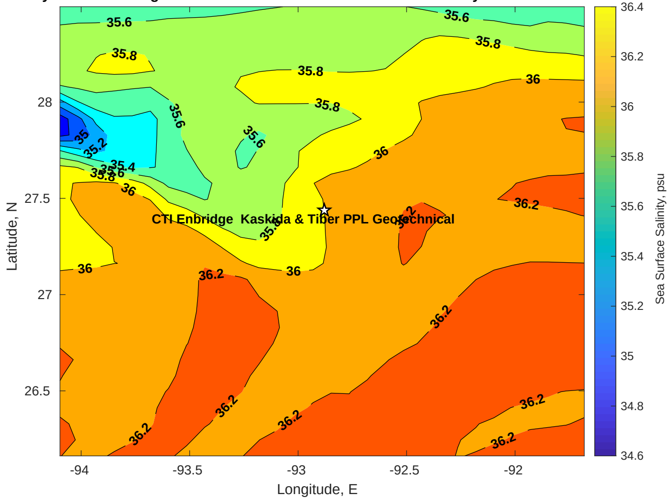
Surface Salinity for CTI Enbridge Kaskida & Tiber PPL Geotechnical at 09-May-2025 00:00:00
