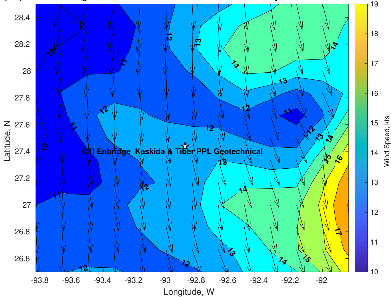
Winds (kts) for CTI Enbridge Kaskida & Tiber PPL Geotechnical at 10-May-2025 09:00:00
