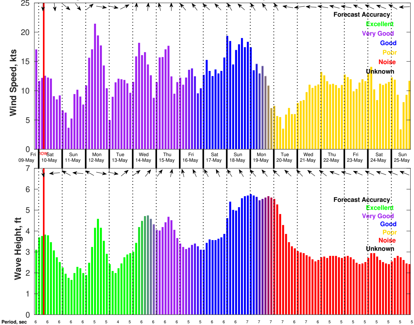
Wind & Wave Forecast for CTI Enbridge Kaskida & Tiber PPL Geotechnical from 09-May-2025 20:00:00 to 25-May-2025 20:00:00
