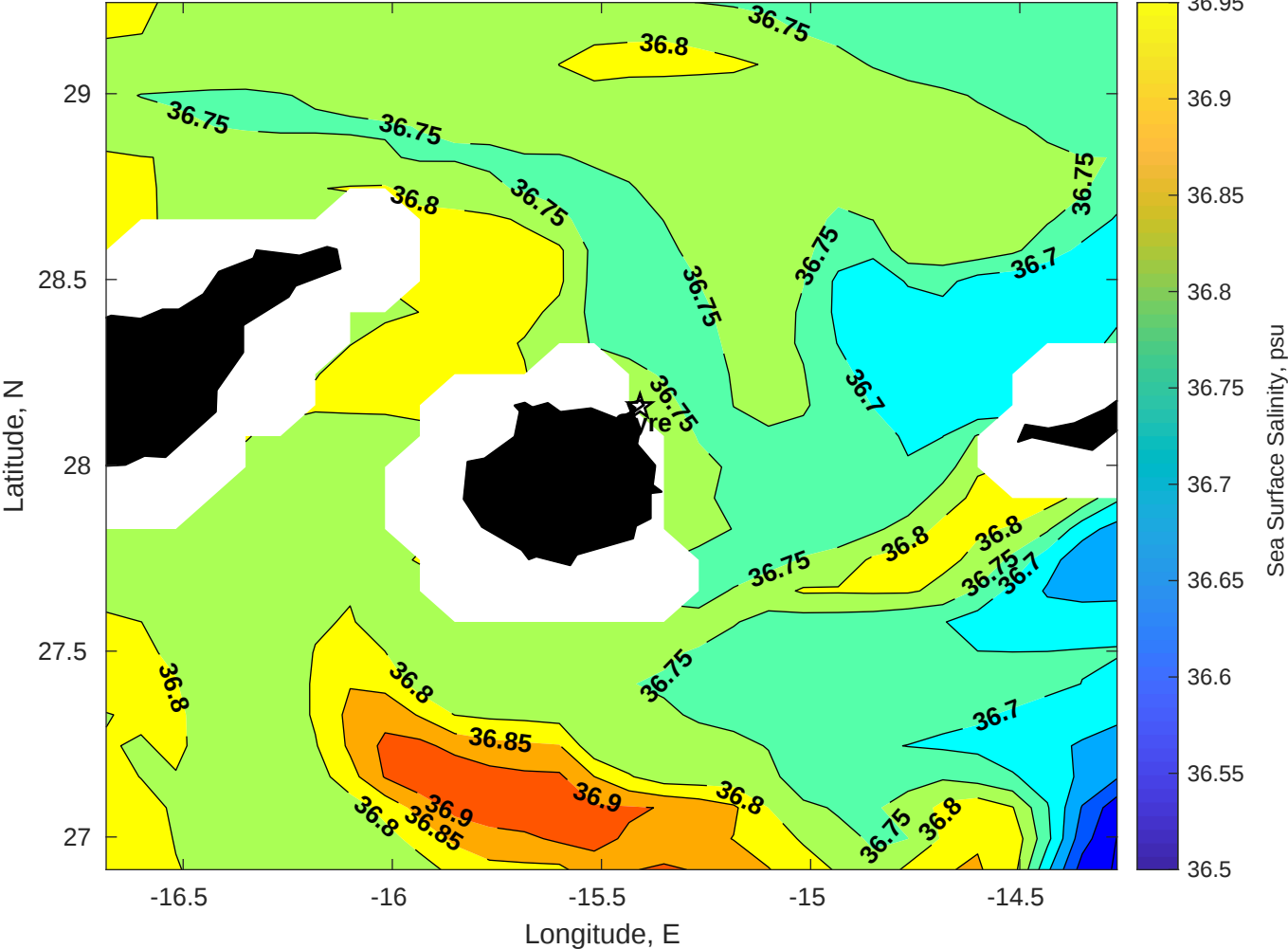
Surface Salinity for Gyre at 09-May-2025 00:00:00
