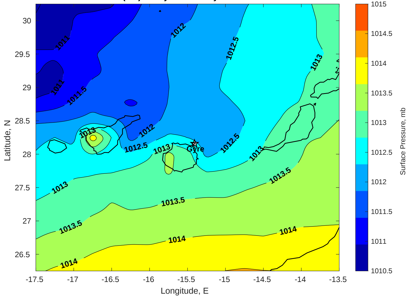
Surface Pressure (mb) for Gyre at 10-May-2025 00:00:00
