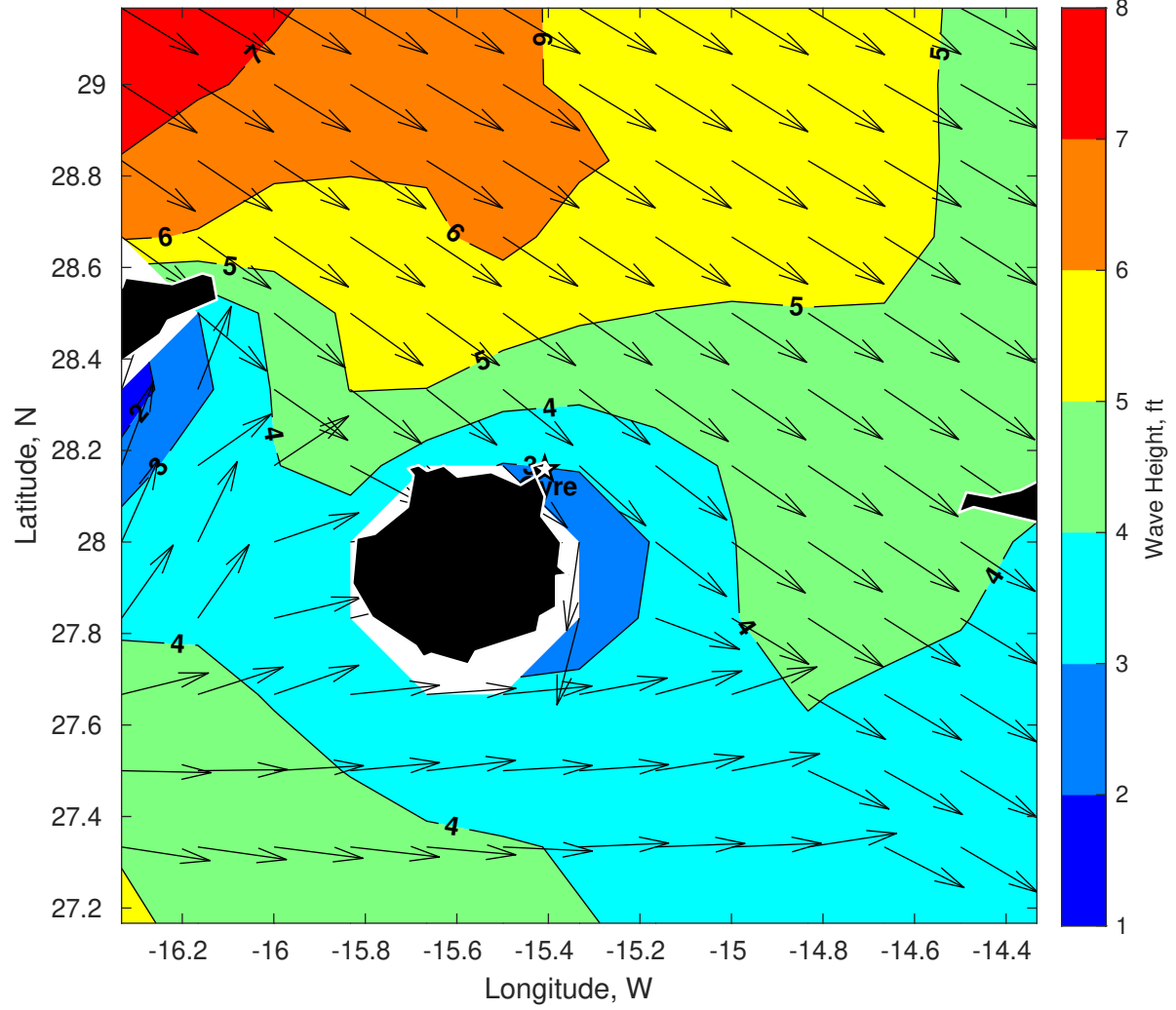
Wave Height (ft) for Gyre at 10-May-2025 09:00:00
