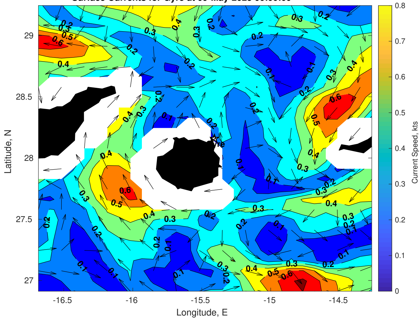
Surface Currents for Gyre at 09-May-2025 00:00:00
