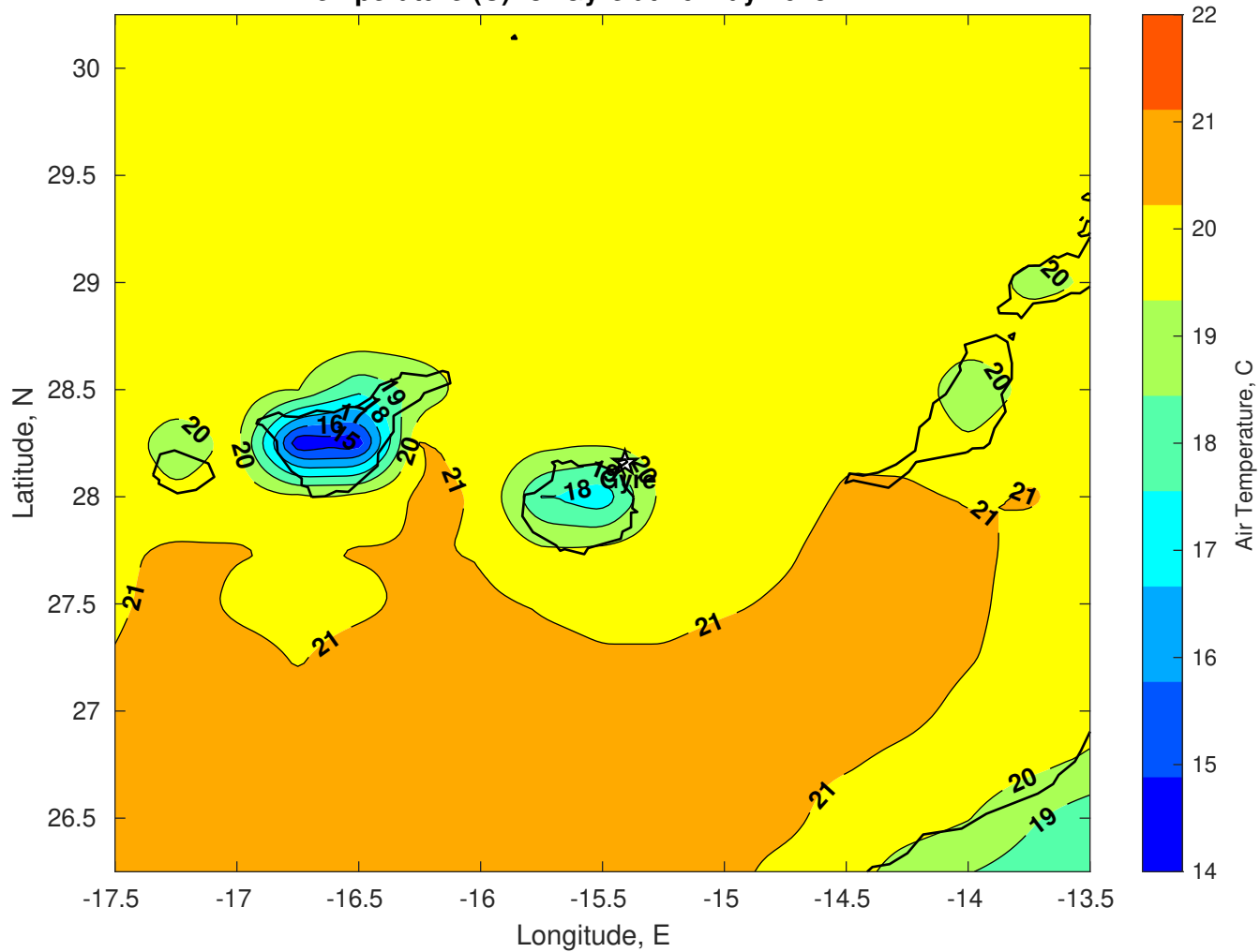
Air Temperature (C) for Gyre at 10-May-2025
