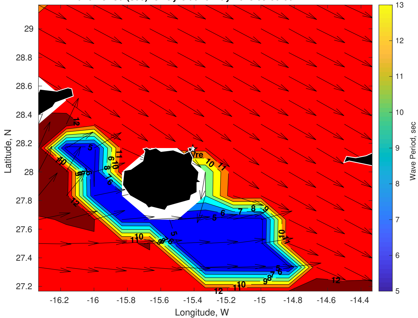
Wave Period (sec) for Gyre at 10-May-2025 09:00:00
