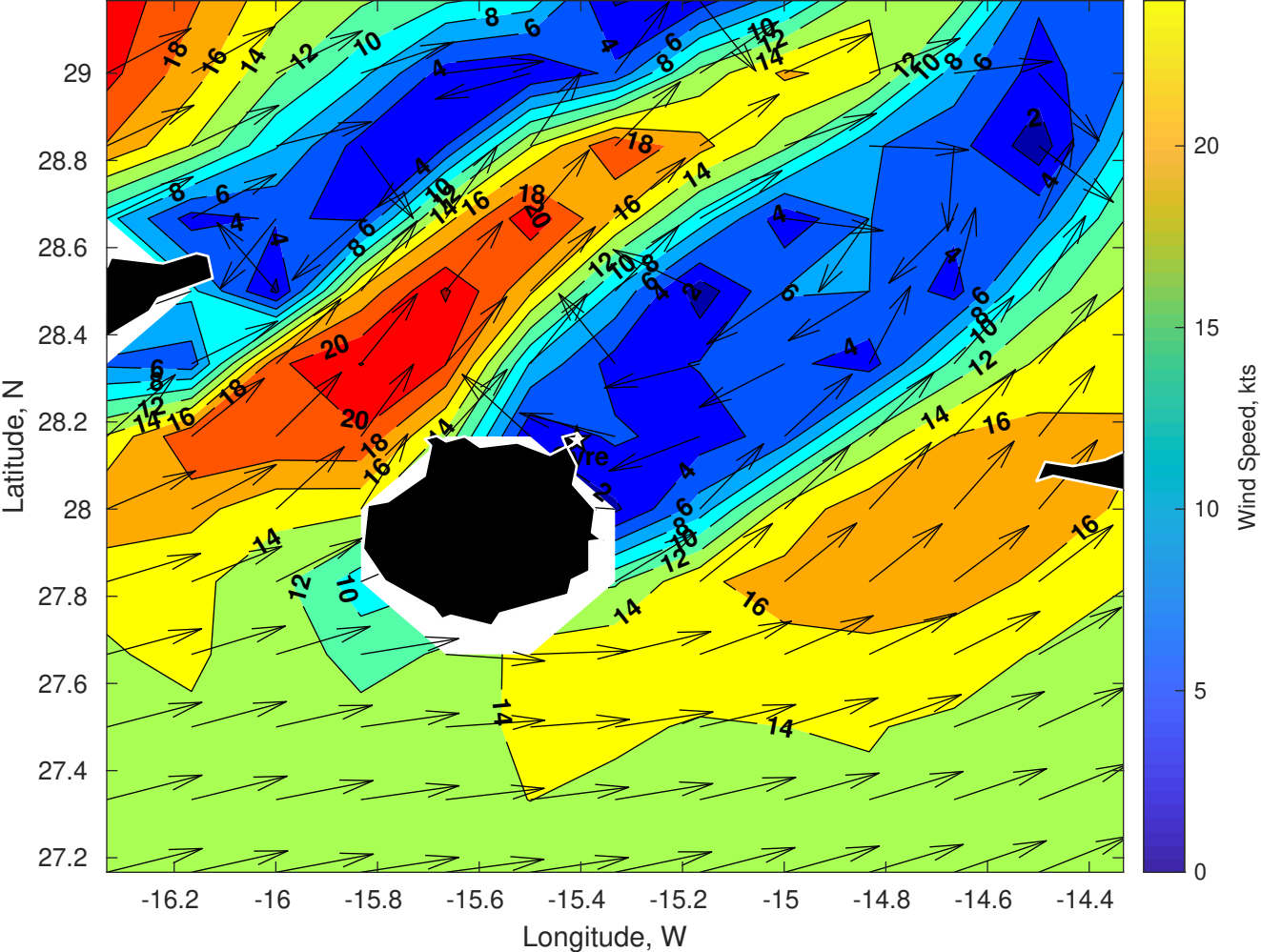
Winds (kts) for Gyre at 10-May-2025 09:00:00
