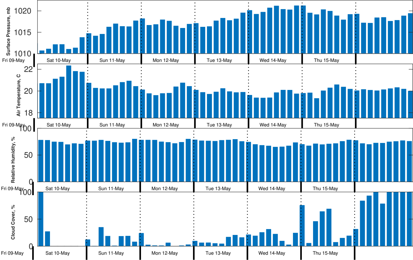
Met Forecast for Gyre from 09-May-2025 23:00:00 to 16-May-2025 23:00:00
