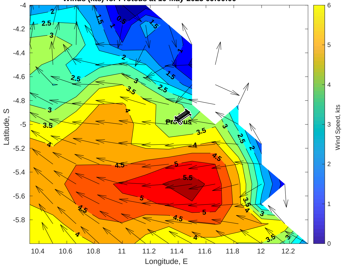
Winds (kts) for Proteus at 10-May-2025 09:00:00
