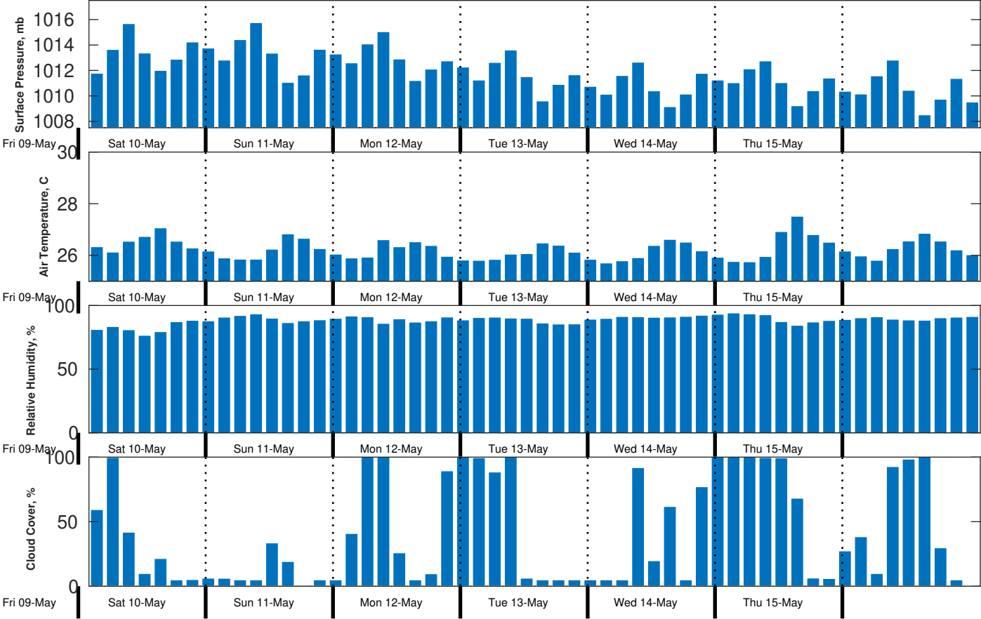
Met Forecast for Proteus from 10-May-2025 00:00:00 to 17-May-2025 00:00:00
