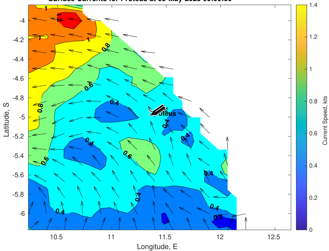
Surface Currents for Proteus at 09-May-2025 00:00:00
