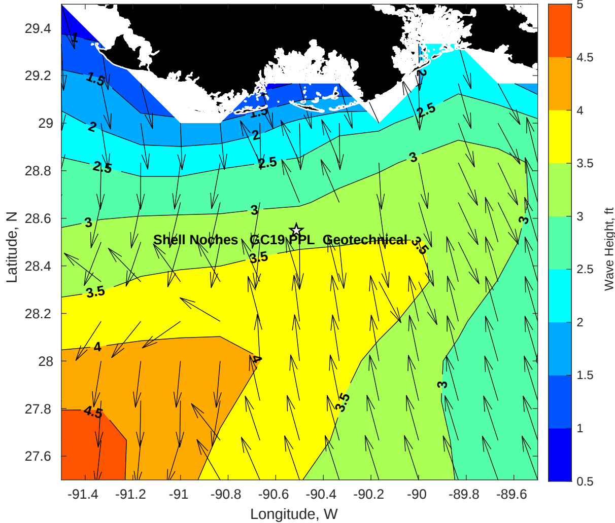
Wave Height (ft) for Shell Noches GC19 PPL Geotechnical at 10-May-2025 09:00:00
