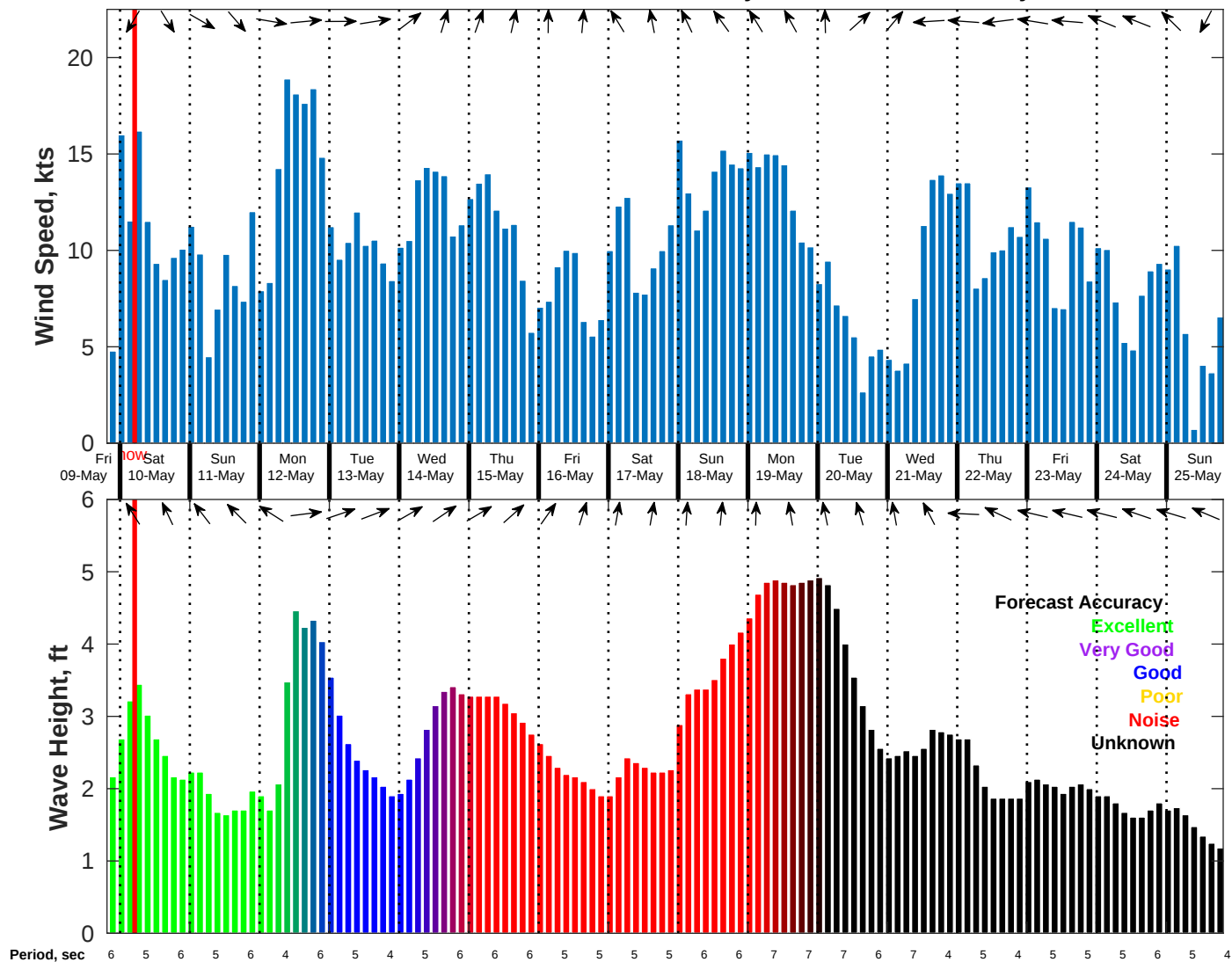
Wind & Wave Forecast for Shell Noches GC19 PPL Geotechnical from 09-May-2025 20:00:00 to 25-May-2025 20:00:00
