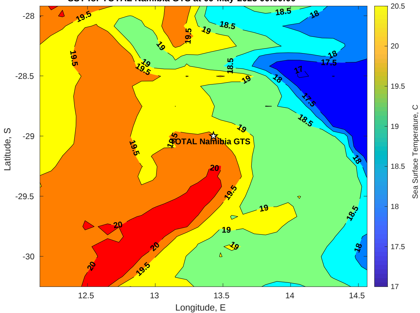
SST for TOTAL Namibia GTS at 09-May-2025 00:00:00
