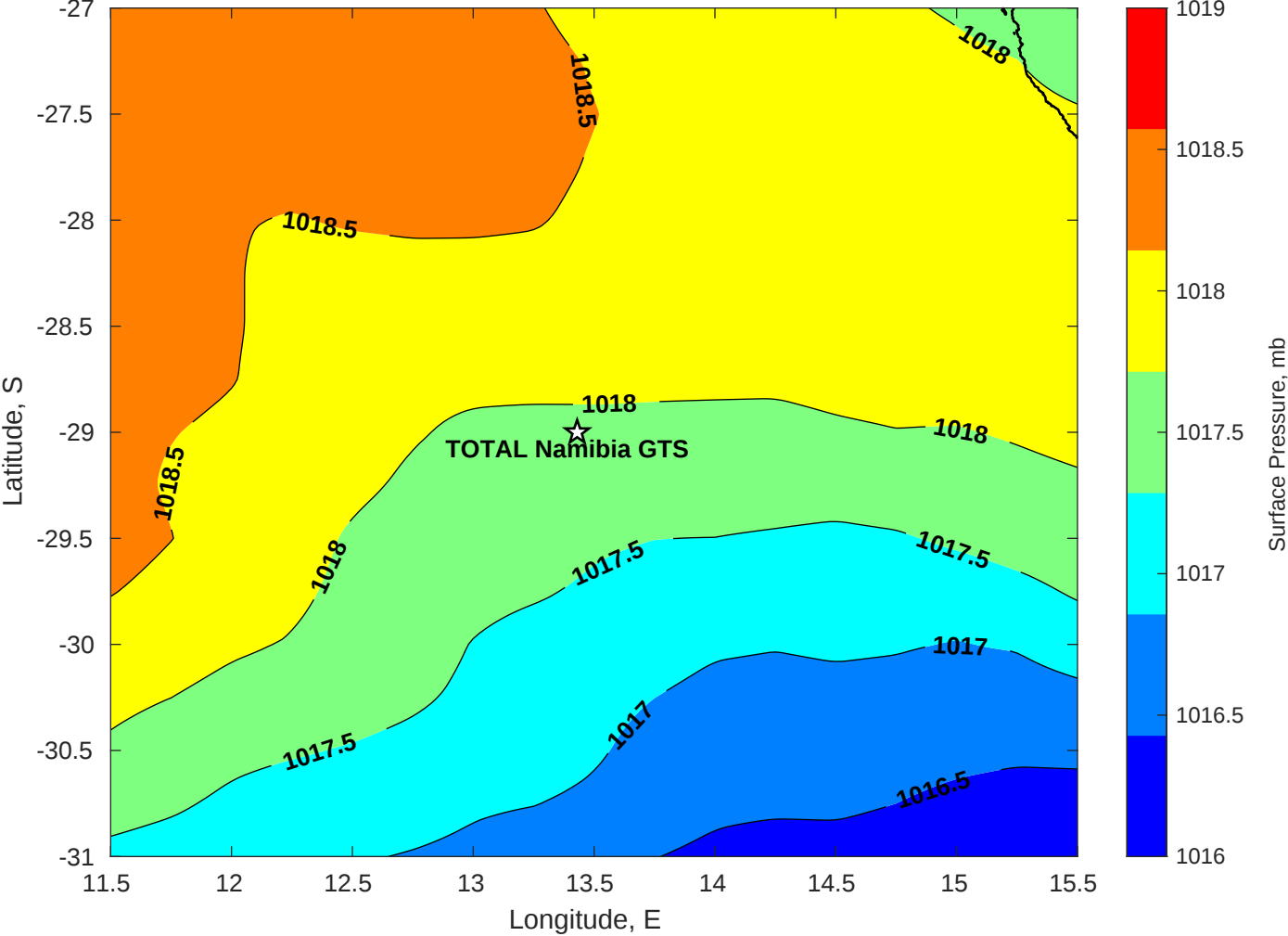
Surface Pressure (mb) for TOTAL Namibia GTS at 10-May-2025 00:00:00
