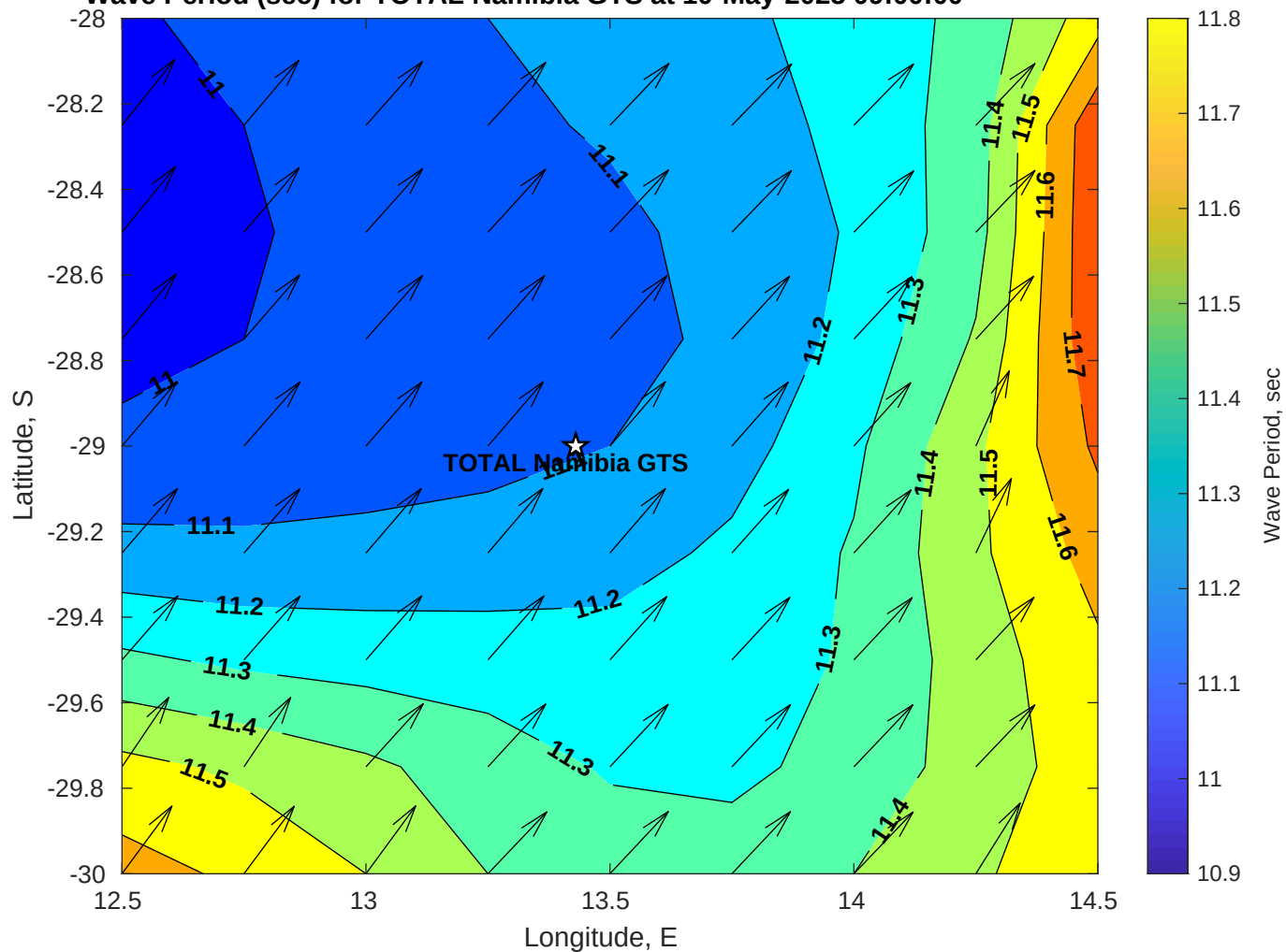
Wave Period (sec) for TOTAL Namibia GTS at 10-May-2025 09:00:00
