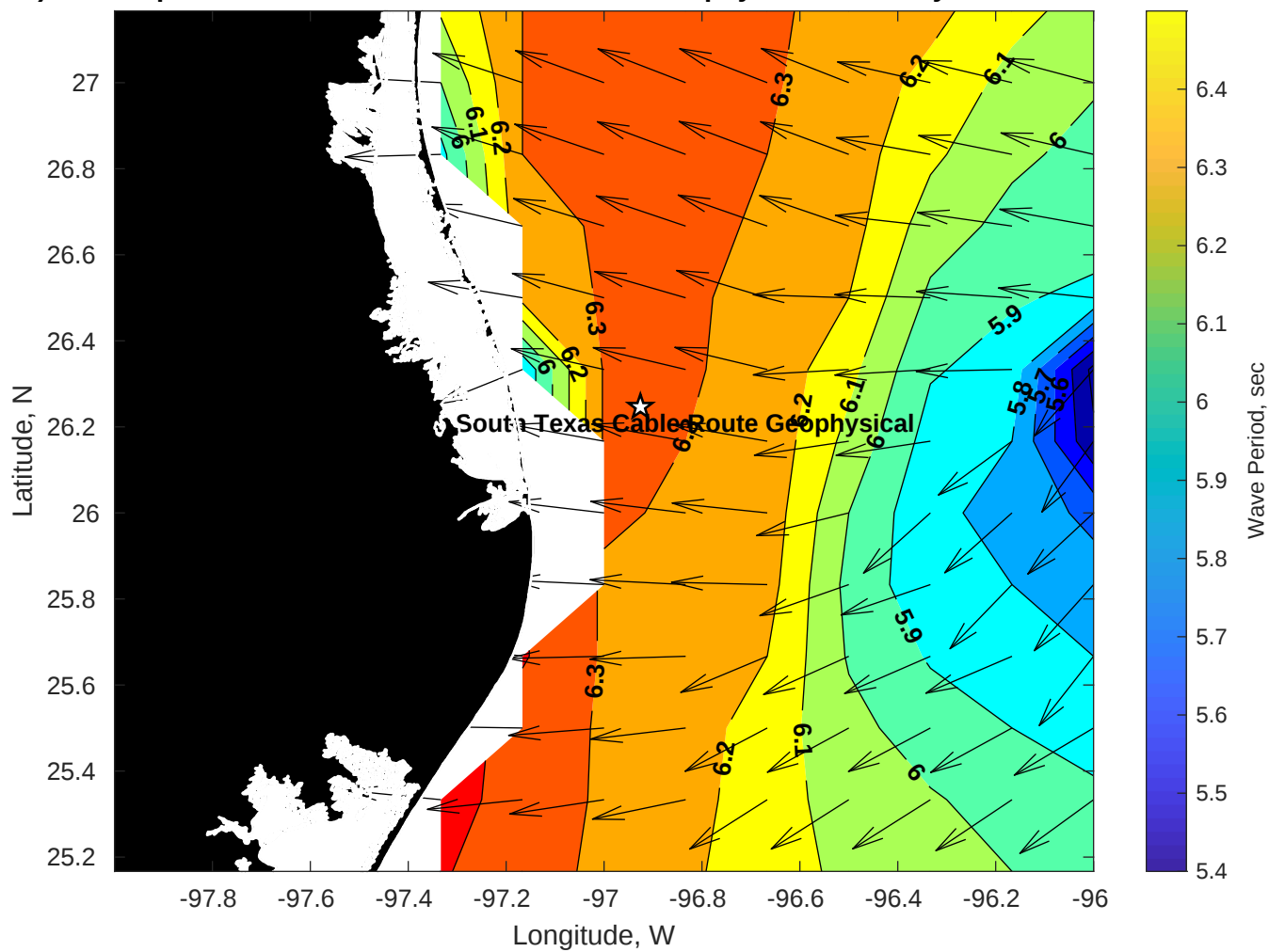
Period (sec) for Tampnet P2378 South Texas Cable Route Geophysical at 10-May-2025 09:00:00
