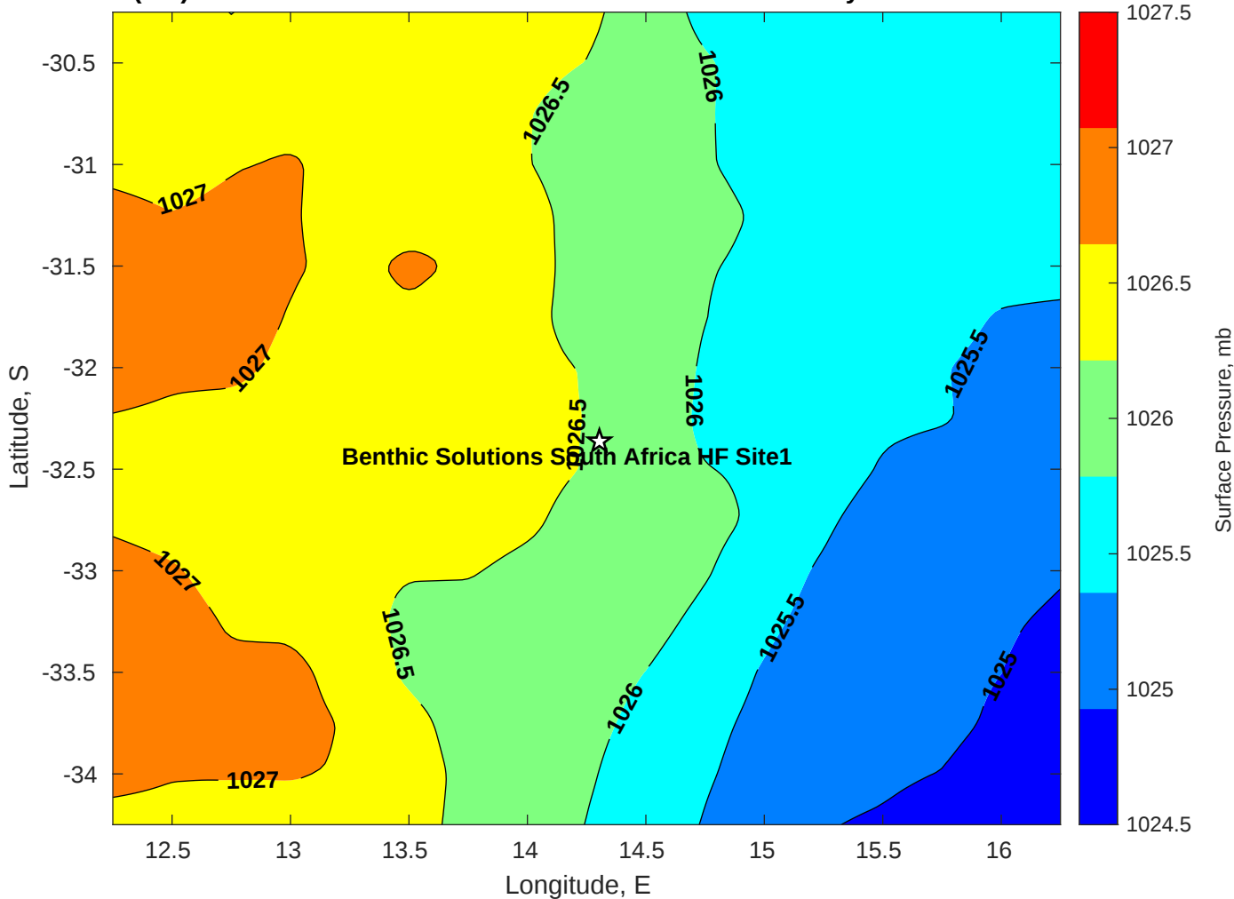
Surface Pressure (mb) for Benthic Solutions South Africa HF Site1 at 11-May-2025 00:00:00
