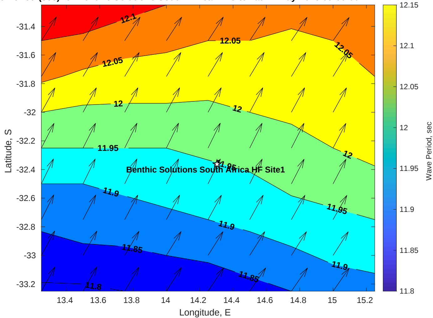
Wave Period (sec) for Benthic Solutions South Africa HF Site1 at 11-May-2025 09:00:00
