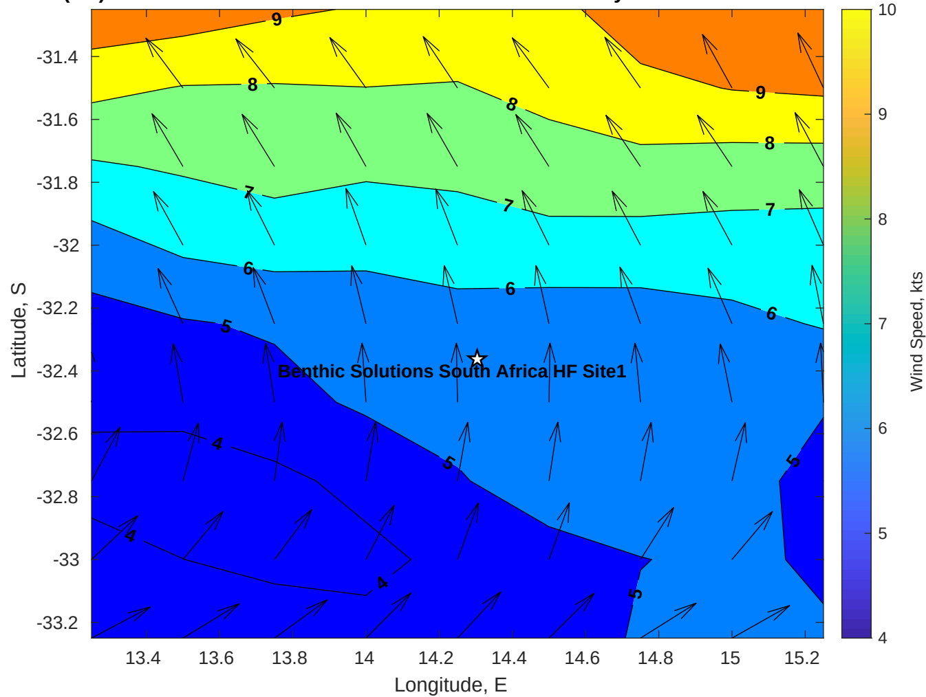
Winds (kts) for Benthic Solutions South Africa HF Site1 at 11-May-2025 09:00:00
