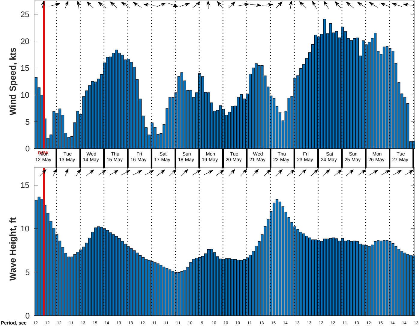
Wind & Wave Forecast for Benthic Solutions South Africa HF Site1 from 11-May-2025 02:00:00 to 27-May-2025 02:00:00
