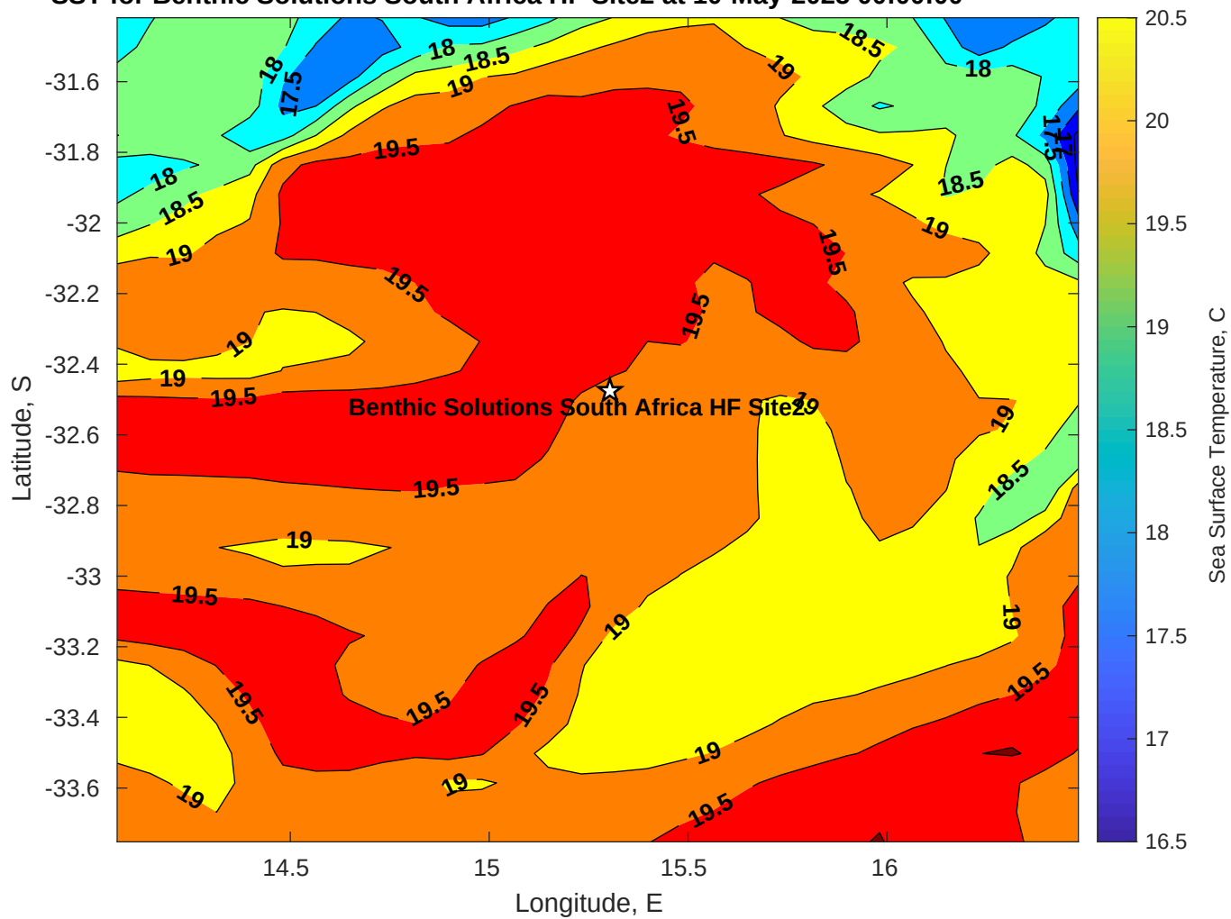
SST for Benthic Solutions South Africa HF Site2 at 10-May-2025 00:00:00
